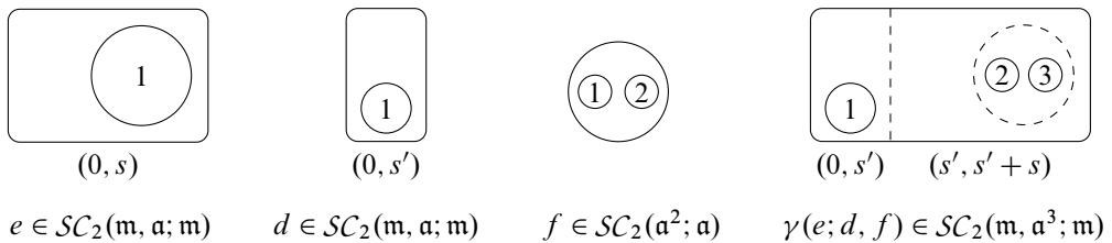
Figure 1: The operadic composition of \mathcal{SC}_n .
