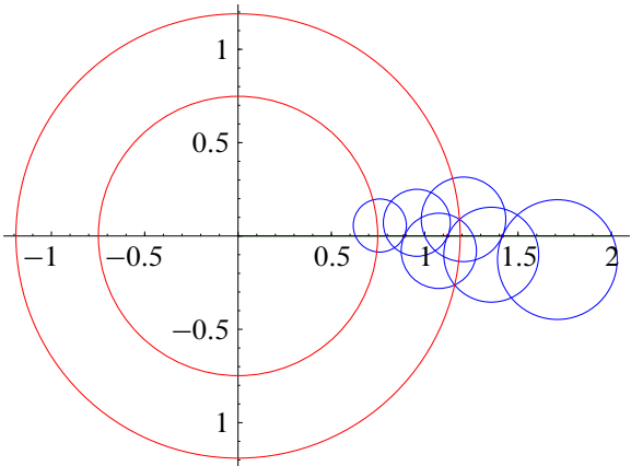
Figure 12: The disks D_k^\pm (in blue) for \alpha_2 = 0.91 .
