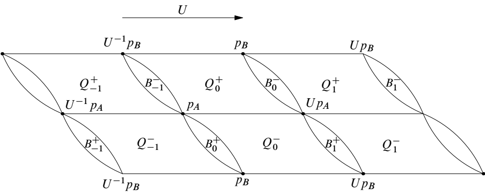
Figure 8: Combinatorics of the boundary at infinity of the Ford domain after the involution. The two horizontal boundaries are identified by a vertical translation.
