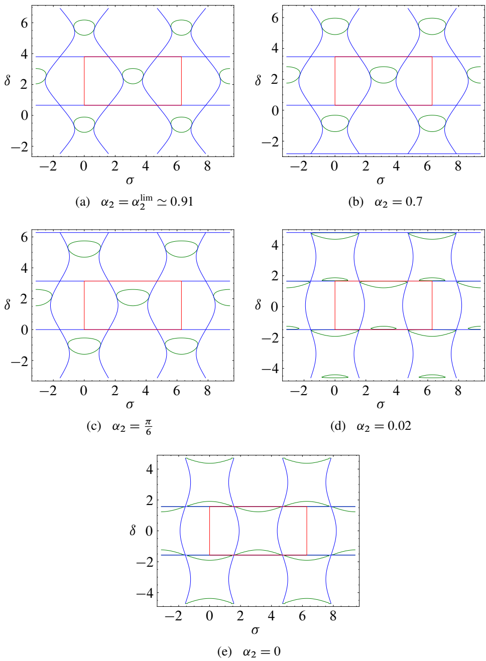
Figure 9: The curves of equations (1) and (2) (blue), the curve of the intersection with \partial_\infty \mathbb{H}^2_{\mathbb{C}} (green) and the rectangle of study (red) for \alpha_2 \in \{0, 0.02, \frac{\pi}{6}, 0.7, \alpha_2^{\text{lim}}\} .
