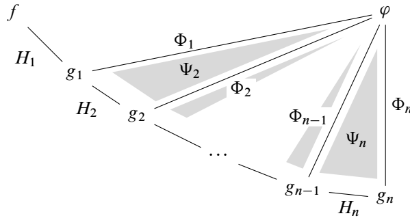
Figure 1: A summary of the various maps, homotopies and second-order homotopies produced in the proof of Theorem 4.1. The bottom row consists of genuine maps X \rightarrow Y and homotopies between them; the rest is on the level of DGAs. Maps become better controlled from left to right.
