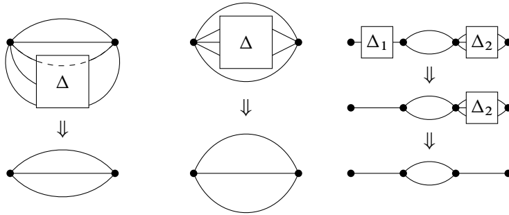
Figure 17: Surgeries for the proof of Lemma 4.16.
