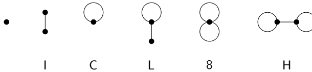
Figure 2: Homeomorphism types of connected small graphs.
