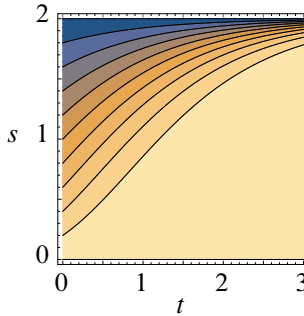
Figure 20: The homotopy of Construction 5.10.
