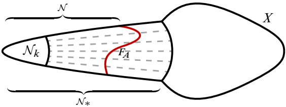
Figure 1: Hypersurface defined by F_A .
