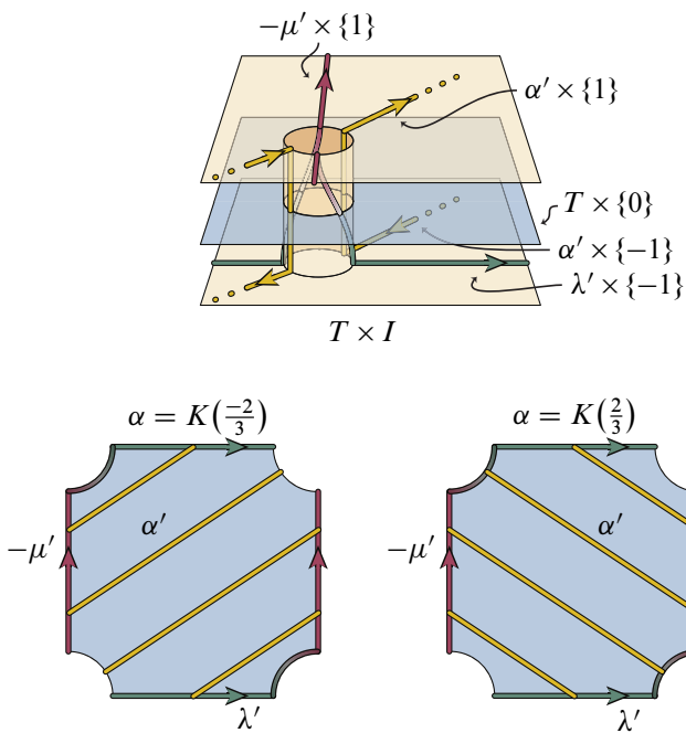
Figure 12: The curve \partial D_\alpha is the union of the two arcs \alpha' \times \{\pm 1\} and two vertical arcs in \partial T \times I since D_\alpha = \alpha' \times I ; in the cylinder \partial T \times I , the curves C_v and \partial D_\alpha are either disjoint or intersect twice; with \alpha of negative slope as shown, they are disjoint (top). The projection of C_v and \partial D_\alpha to T where \alpha = K(a_1/a_2) is illustrated for negative slopes with a_1/a_2 = -\frac{2}{3} (bottom left) and for positive slopes with a_1/a_2 = \frac{2}{3} (bottom right).
