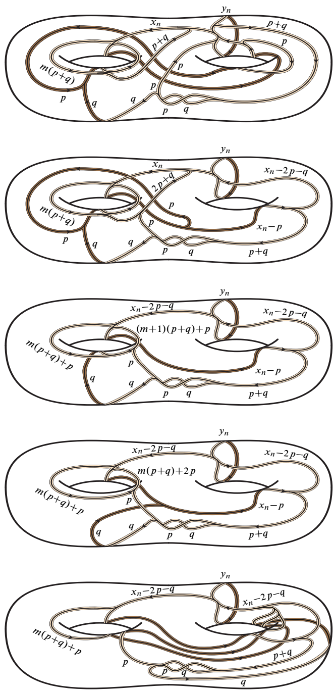
Figure 26a: A sequence of isotopies (continued in Figure 26b) shows the framed train track of Figure 25 carries closed positive braids.
