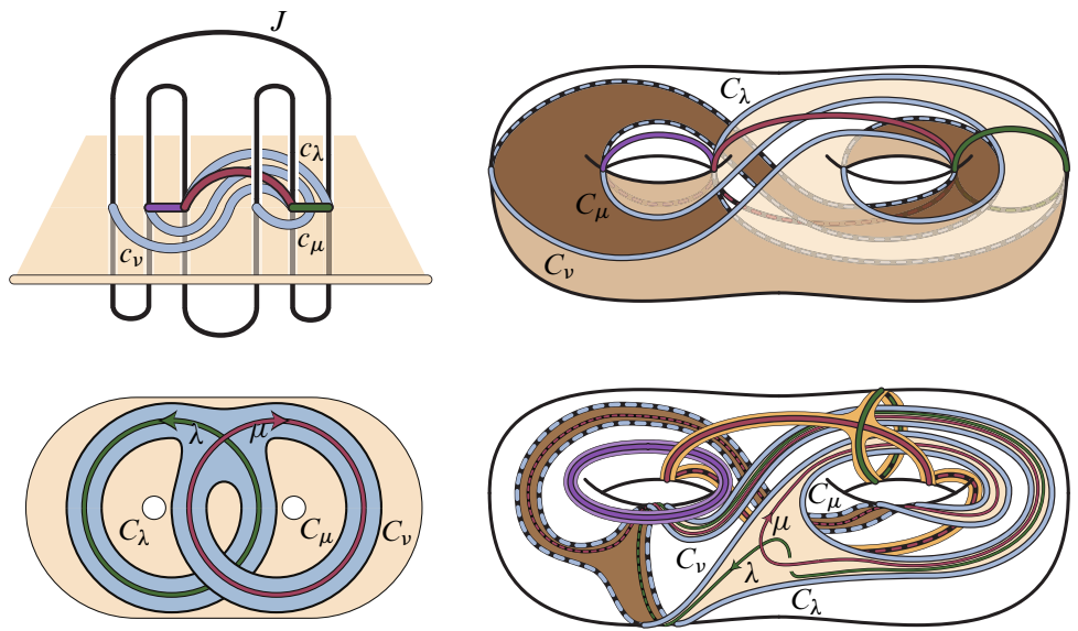
Figure 24: The double branched cover of the planar 3–bridge unknot gives a genus 2 Heegaard surface containing the lifts of the arcs in the bridge sphere (top, left and right). After an isotopy, the curves C_v , C_\mu , and C_\lambda more clearly bound the pair-of-pants P (bottom right). The basis of curves \mu and \lambda in the once-punctured torus T are shown in P . Figure 2 (bottom left) is included for reference.
