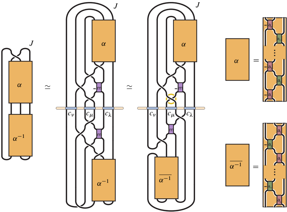
Figure 7: A diagram of the unknot J = J^{\alpha,m} in a 3-bridge position so that it is almost-alternating when m \geq 0 and a_i \geq 0 for i = 1, 2, \dots, n is shown in the middle. The dealternating crossing is circled.
