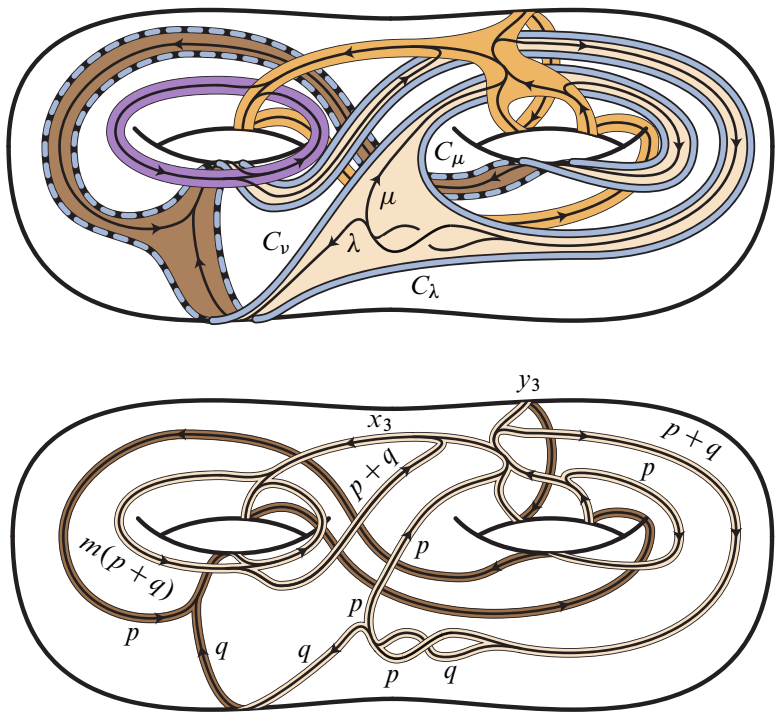
Figure 25: The p/q -lashing of P (for p, q > 0 ) as a framed train track in the Heegaard surface. Here m \geq 0 and \alpha = \sigma_1^{-a_3} \sigma_2^{a_2} \sigma_1^{-a_1} , where a_1, a_2, a_3 \geq 0 are such that x_3 = ((a_3 a_2 (a_1 + 2) + a_3 + a_1 + 2)(m + 2) - 2a_3 a_2)p + ((a_3 a_2 (a_1 + 2) + a_3 + a_1 + 2)(m + 1) - a_3 a_2)q and such that y_3 = (a_2 (a_1 + 2)(m + 2) - 2a_2)p + (a_2 (a_1 + 2)(m + 1) - a_2)q .
