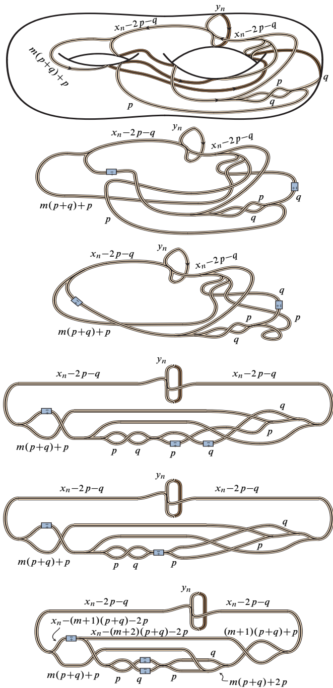
Figure 26b: A sequence of isotopies (continued from Figure 26a) shows the framed train track of Figure 25 carries closed positive braids.
