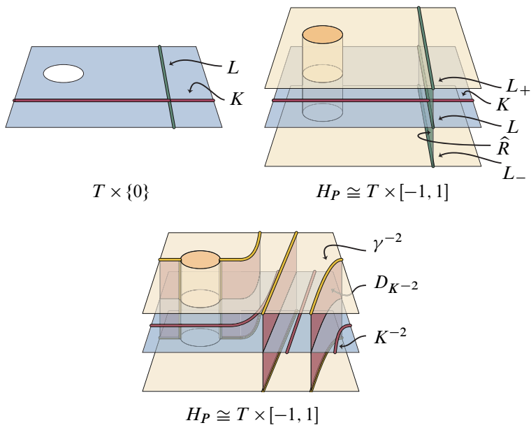
Figure 10: Up to homeomorphism, the curves K and L appear in T as shown (top left); opposite sides of the figure are identified. In H_P \cong T \times [-1, 1] , the curve L defines an annulus \hat{R} with boundary L_+ \cup L_- (top right). We twist K and D_K twice to the left along L and \hat{R} to produce the curve K^{-2} and the disk D_{K^{-2}} (bottom).
