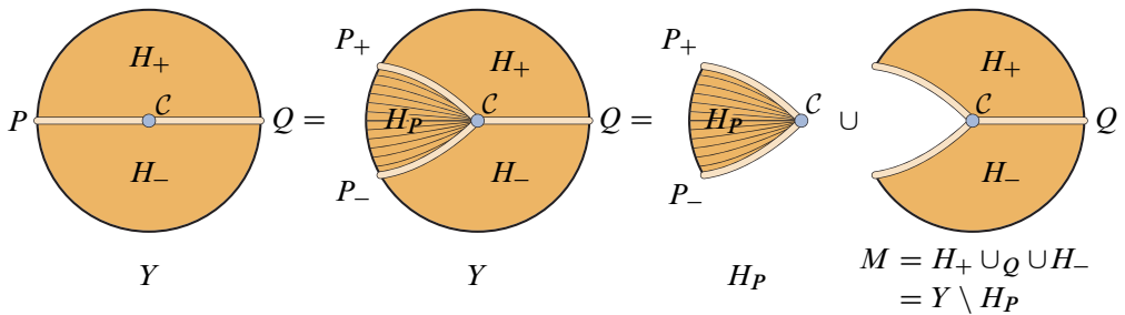
Figure 14: The schematic decomposition of Y along the three pairs of pants P_+ , P_- , and Q .
