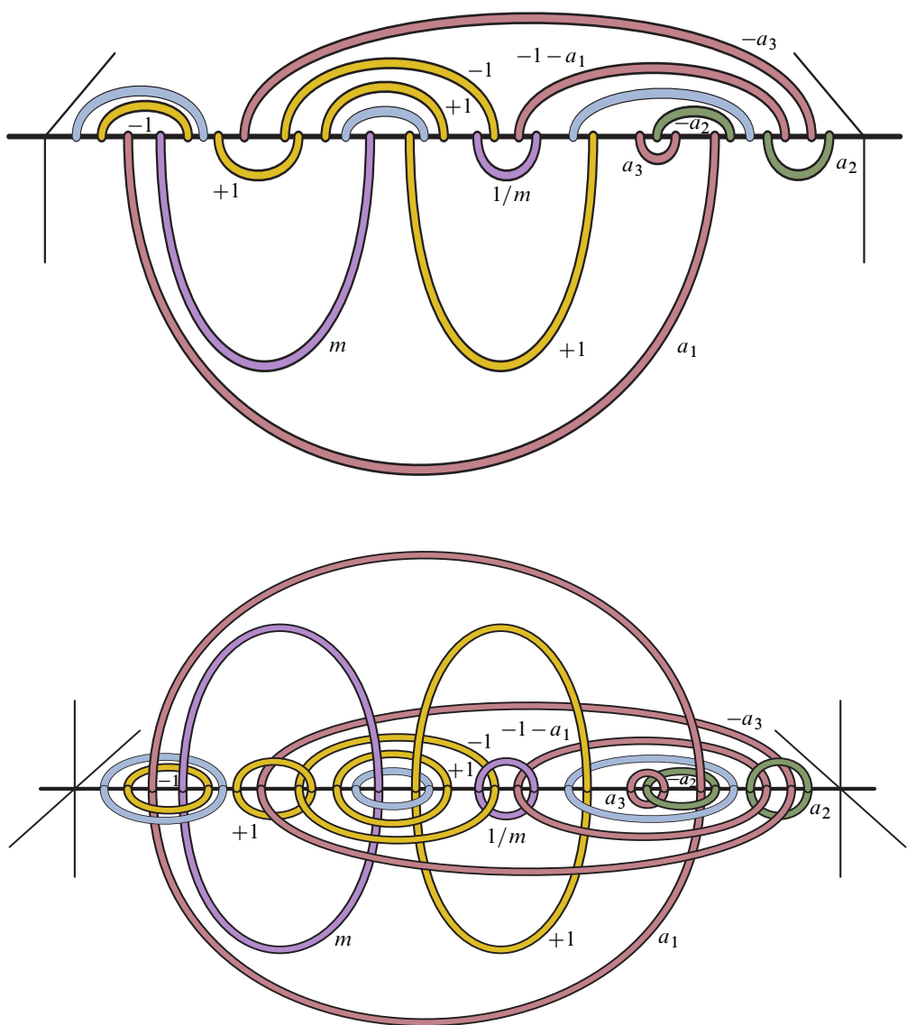
Figure 21: The planar unknot at the end of Figure 20 is mapped to a horizontal axis (with a point at infinity) so that its inside becomes a horizontal half-plane into the page while its outside becomes a downward vertical half-plane (top). This facilitates the visualization of the lifts of the arcs in the double cover of S^3 branched over the unknot (bottom). The rational tangle replacement instructions lift to Dehn surgery instructions and the arcs c_\nu , c_\mu , and c_\lambda lift to the knots C_\nu , C_\mu , and C_\lambda .
