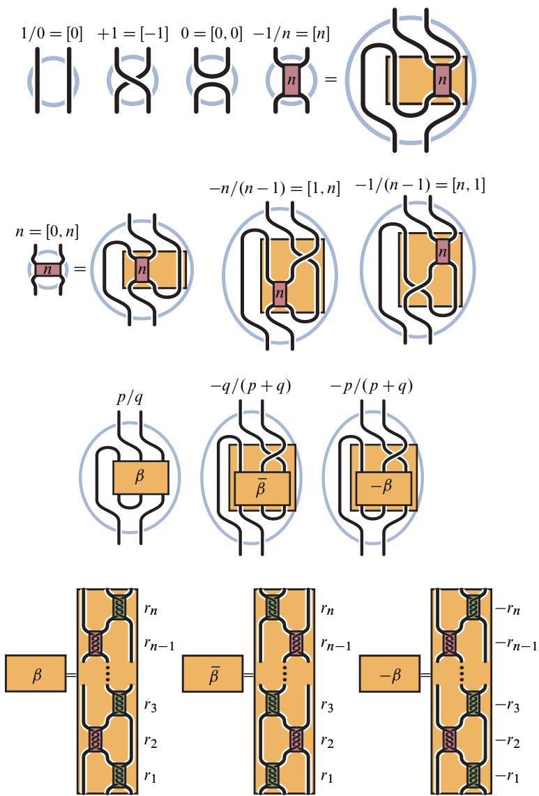
Figure 6: The top two rows show the convention for continued fractions and the corresponding rational tangles. (A twist box labeled n means n vertical right-handed twists when n > 0 and |n| vertical left-handed twists when n < 0 .) The bottom two rows indicate the general forms for the related rational tangles of slopes p/q , -q/(p+q) , and -p/(p+q) , where, for n odd, p/q = [r_n, \dots, r_2, r_1] , -q/(p+q) = [1, r_n, r_{n-1}, \dots, r_2, r_1] , and -p/(p+q) = [1-r_n, -r_{n-1}, \dots, -r_2, -r_1] . As illustrated, when r_i \leq 0 for i odd and r_i \geq 0 for i even, these tangles are alternating.
