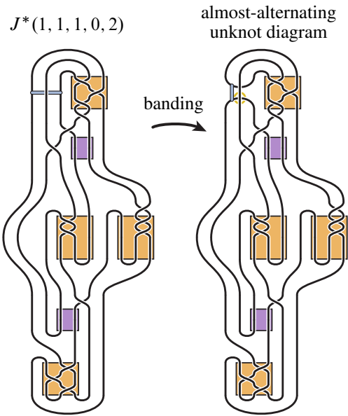
Figure 29: The alternating knot J^*(1, 1, 1, 0, 2) admits a banding along an arc that crosses an alternating diagram once to produce an almost-alternating diagram of the unknot.
