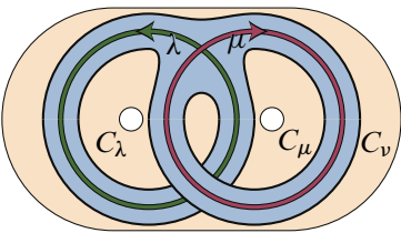
Figure 2: A projection to P of the once-punctured torus T \subset P \times I with its basis of curves \mu and \lambda along with the three boundary curves C_v , C_\mu , and C_\lambda .
