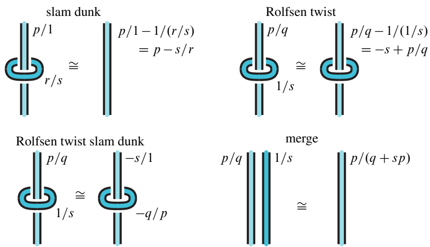
Figure 4: A few basic moves on surgery diagrams. The merge move amalgamates two surgery curves cobounding an annulus along their 0-framings.
