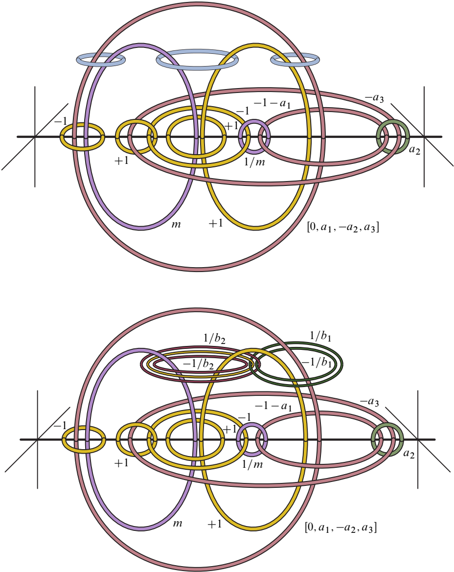
Figure 22: The genus 2 Heegaard surface containing the knots C_v , C_\mu , and C_\lambda can be traced through its lift of the bridge sphere at the beginning of Figure 20 (top). Here we lift these curves upwards to recognize the punctured horizontal plane they bound (with the point at infinity) as the pair of pants P in which our lashings occur. This triple of knots is then traded for the interlaced stack of knots as in Figure 5 to give surgery instructions for a p/q -lashing (bottom). Recall the convention p/q = [-b_n, b_{n-1}, \dots, b_2, -b_1] with b_j \geq 0 .
