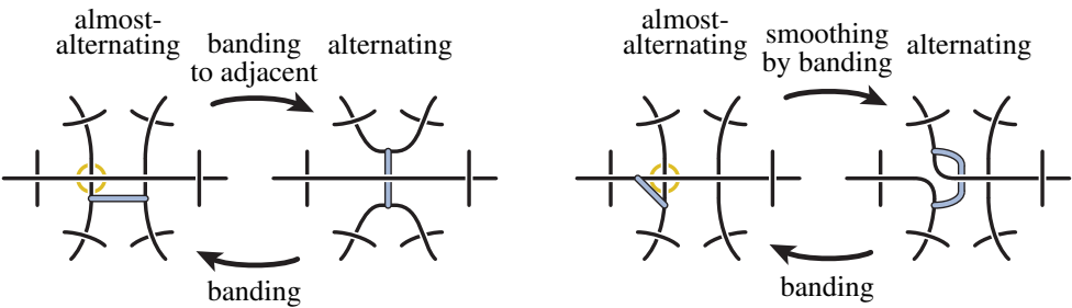
Figure 31: In an almost-alternating diagram, a banding of the dealternation crossing to an adjacent crossing produces an alternating diagram (left). The dual blackboard framed arc in the alternating diagram crosses the diagram once. In an almost-alternating diagram, a smoothing of the dealternation crossing by a banding is shown, though the intermediate removal of a nugatory crossing is not shown (right). The dual blackboard framed arc in the alternating diagram is shown.
