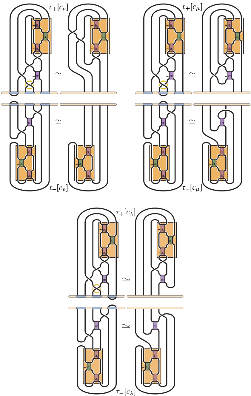
Figure 16: Shown in the case that n = 3 , the tangles resulting from the arc-closures of the tangles \tau_+ and \tau_- along the components of c individually are isotoped to simpler, alternating diagrams.
