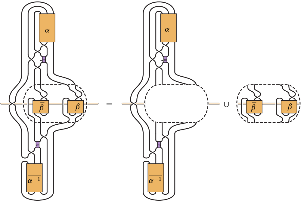
Figure 19: The link J_c^{\alpha,m}(+1, -q/(p+q), -p/(p+q)) splits into two 4-strand tangles as shown. One fairly easily sees that each of these two tangles is freely isotopic to the trivial 4-strand tangle.
