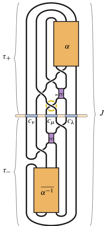
Figure 15: The knot J = J^{\alpha,m} from the center of Figure 7 is shown again, divided into the tangles \tau_+ and \tau_- .
