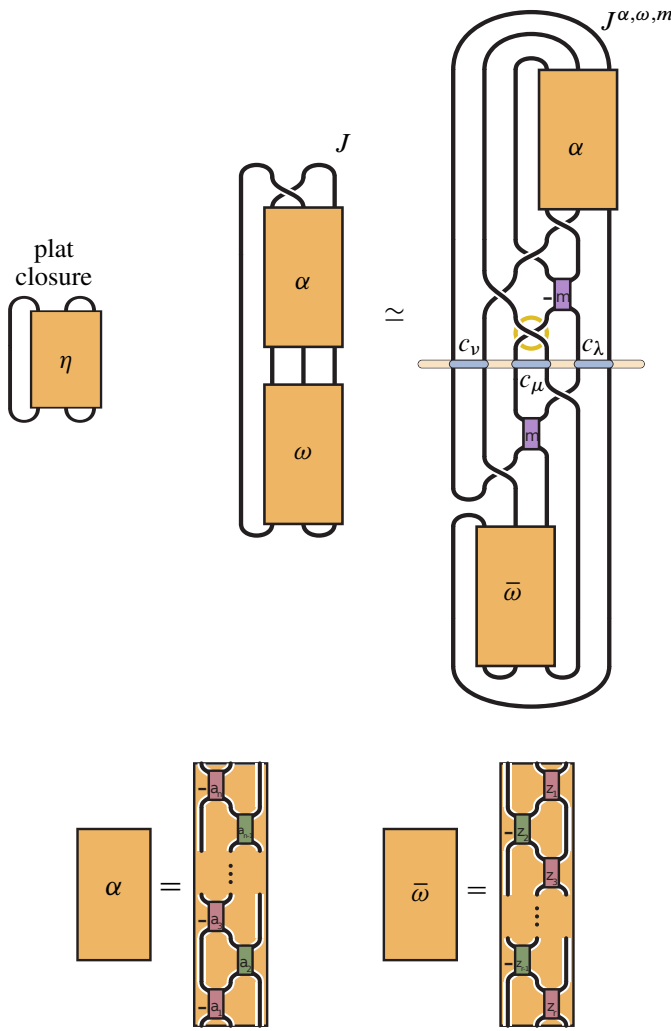
Figure 18: The plat closure of a 3–braid \eta (top left). Replacing \alpha^{-1} in Figure 7 with another braid \omega enables the production of almost-alternating diagrams J^{\alpha, \omega, m} of other 2–bridge links, analogous to our almost-alternating unknot diagrams (top right). The braids \alpha and \bar{\omega} are shown for \alpha and \omega in form (*) with n and r odd (bottom).
