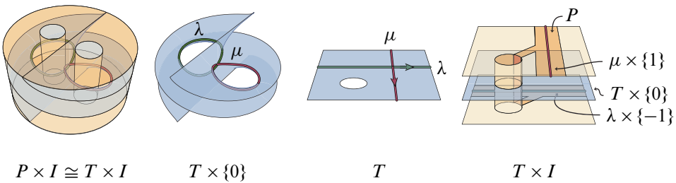
Figure 3: The handlebody P \times I (\cong T \times I) containing the properly embedded once-punctured torus T = T \times \{0\} , along with this configuration of T \times \{0\} isolated and the curves \lambda and \mu labeled (leftmost two). The once-punctured torus T and its curves \lambda and \mu in a more standard form where opposite sides of the rectangle are identified (second from right). On the far right is a view of the handlebody T \times I (\cong P \times I) with the pair of pants P = P \times \{1\} marked on its boundary. (This figure is essentially Figures 1 and 2 from [2] except that \mu and \lambda are swapped. Equivalently, one may change the orientation of T in [2, Figure 2].)
