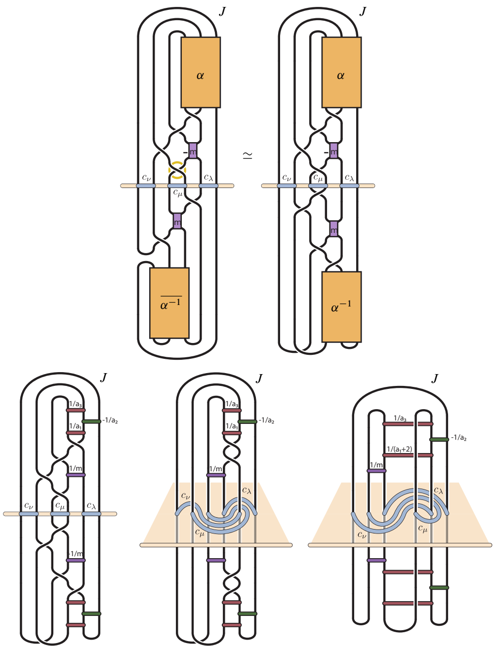
Figure 23: Isotopy, pairs of tangle replacements, and twisting transform the almost-alternating unknot J^{\alpha,m} into a planar 3-bridge unknot where the arcs c_\nu , c_\mu , and c_\lambda are twisted along the bridge sphere.
