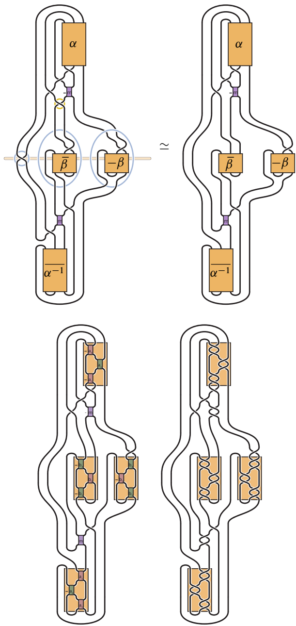
Figure 8: The rational tangle replacements on the link J^{\alpha,m} are made along c to produce the link J_c^{\alpha,m}(+1, -q/(p+q), -p/(p+q)) and then the diagram is simplified to be alternating. Examples with \alpha and \beta of length 3 and further with m = a_1 = a_2 = a_3 = b_1 = b_2 = b_3 = 2 are shown.
