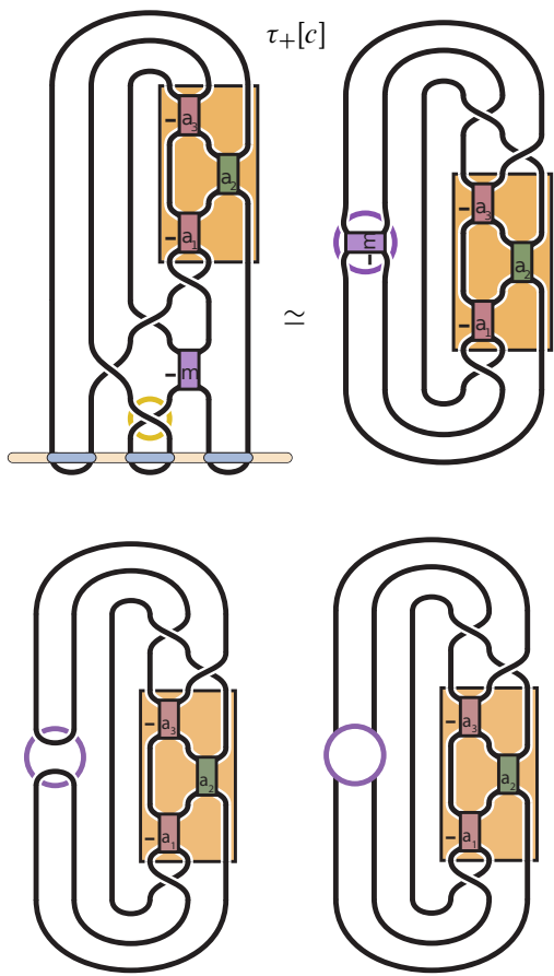
Figure 17: The c -closure of \tau_+ is simplified to a reduced, prime, alternating link (top). A rational tangle replacement of distance \Delta = m produces a 2-bridge link with a nonsplit reduced alternating diagram (bottom left). The exterior of the -m -twist tangle is the tangle \chi , shown with a reduced alternating diagram (bottom right).
