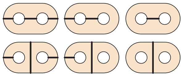
Figure 13: Enumerated are the six possible configurations, up to homeomorphism, of the nonempty set of arcs R \cap R' in the pair of pants R' such that the arcs are essential in R' and no two are parallel.
