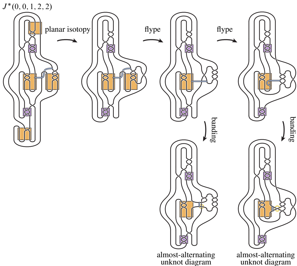
Figure 30: The alternating knot J^*(0, 0, 1, 2, 2) , after planar isotopy and a flype, admits a banding along a flat arc crossing an alternating diagram once to produce an almost-alternating diagram of the unknot. After a further flype, this banding is dual to the smoothing of the dealternation crossing in an almost-alternating diagram of the unknot.
