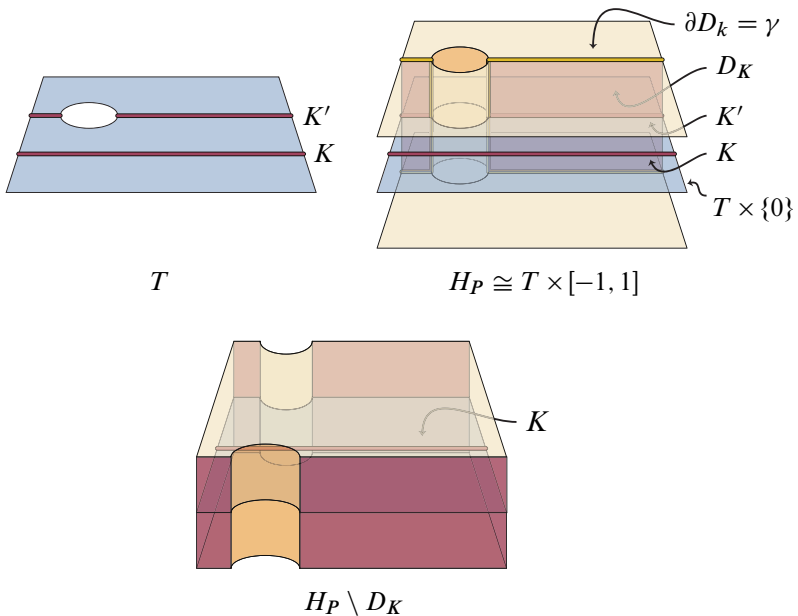
Figure 9: Up to homeomorphism, an essential curve K in T and its associated arc K' (top left); opposite sides of the figure are identified. In H_P \cong T \times [-1, 1] , the arc K' defines a disk D_K with boundary \gamma (top right). Chopping H_P along the disk D_K produces a solid torus in which K is isotopic to the core (bottom); left and right sides of the figure are identified.
