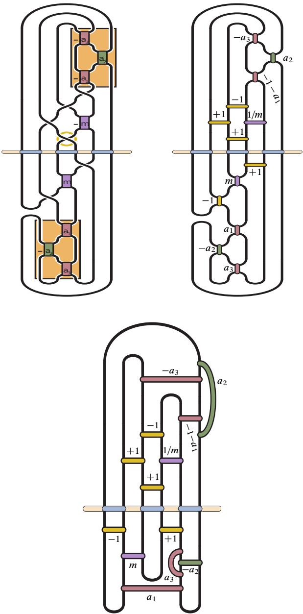
Figure 20: Twist regions (top left) of Figure 7 with the choice \alpha = \sigma_1^{-a_3} \sigma_2^{a_2} \sigma_1^{-a_1} are traded (top right) for blackboard framed arcs with rational tangle replacement instructions. The diagram is then simplified by a planar isotopy that more clearly exhibits the resulting link as a planar unknot while retaining a sense of the original structure (bottom).
