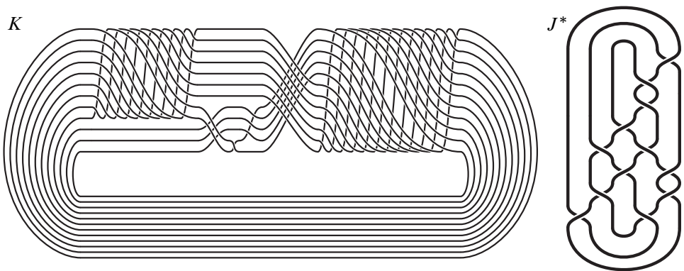
Figure 1: The knot K (left) is the closure of a 12-strand positive braid of length 249. It is an asymmetric hyperbolic L -space knot. The result of 272-surgery on K produces the double branched cover of the 12-crossing alternating link J^* (right).
