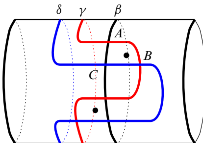
Figure 3: If \delta is obtained from \beta by a Hamiltonian isotopy supported away from the marked points, the domain of the distinguished triangle class in (\Sigma, \beta, \gamma, \delta, z) connecting \Theta_{\beta\gamma} , \Theta_{\gamma\delta} and \Theta_{\beta\delta} will contain one of the marked points corresponding to the strands connected by \mathbb{I} . The intersection of the domain of the triangle with the surface is the small triangle connecting A , B and C .
