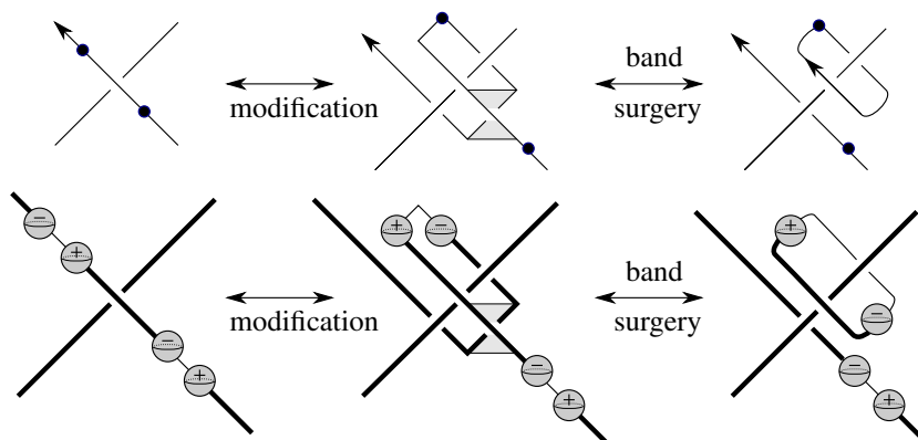
Figure 1: We may change a crossing in the expense of adding a meridian. The meridian can be positively or negatively oriented depending on whether the initial crossing is positive or negative, respectively.
