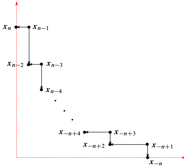
Figure 5: Each horizontal arrow from x_i to x_{i+1} has length a_{i+1} - a_i , while each vertical arrow from x_i to x_{i-1} has length a_i - a_{i-1} .
