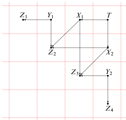
Figure 10: The chain complex C associated with the knot T_{4,5} \# -T_{2,3;2,5} \# T_{2,3} .
