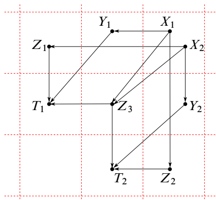
Figure 8: The chain complex associated with the knot T_{2,3;2,-1} .
