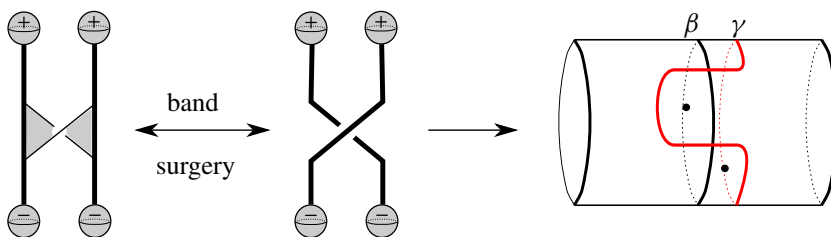
Figure 2: On the right are the two special \beta and \gamma curves corresponding to the band surgery on the Heegaard diagram subordinate to the band.
