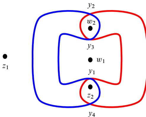
Figure 4: Heegaard diagram for the Hopf link, where the Heegaard surface is S^2 , the red curve is an \alpha curve and the blue curve is a \beta curve.
