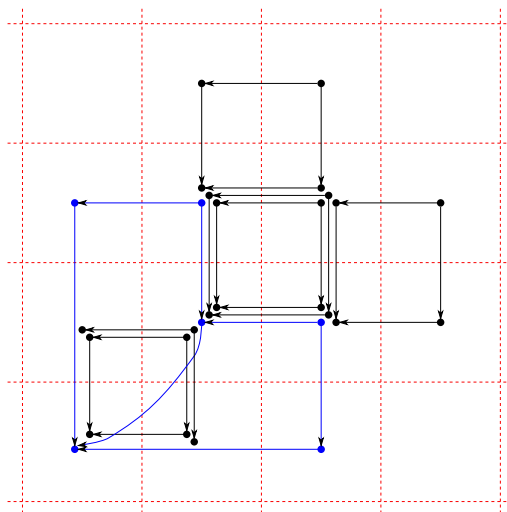
Figure 7: The chain complex associated with the knot 12n_{404} .
