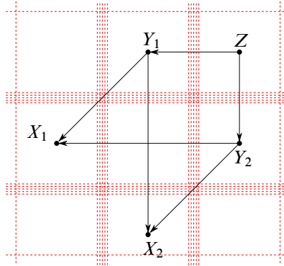
Figure 11: The chain complex C_{i,j} .
