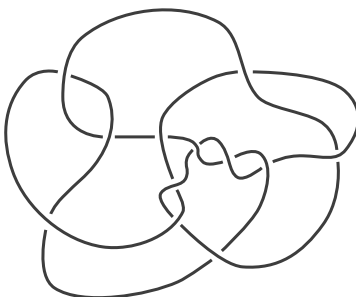
Figure 6: The knot 12n_{404} .
