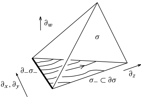
Figure 7: Various parts of \sigma . The thickened line represents \partial_-\sigma_- . The coordinate directions shown are provided, roughly, by the identification of \sigma with a model structure (Section 2.4); this will be proven in Section 6.2.7.
