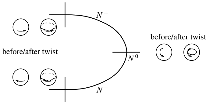
Figure 4: The Engel–Lutz twist in terms of the curves H_p and \lambda_p near a hypersurface N = N^+ \cup N^- \cup N^0 (represented by the U -shaped curve).
