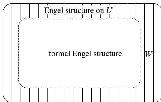
Figure 1: In general one cannot extend every Engel structure from U = \mathcal{Op}(\partial\mathbb{D}^4) to the interior of M = \mathbb{D}^4 using the methods of [2]. The integral lines of the characteristic foliation are depicted as vertical segments.
