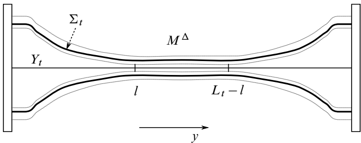
Figure 5: A transverse surface \Sigma_t together with a tubular neighborhood where an Engel–Lutz twist is performed.
