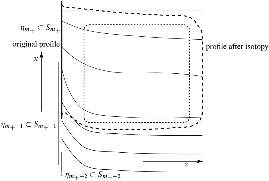
Figure 11: The line field TL \cap \mathcal{D}_1 .
