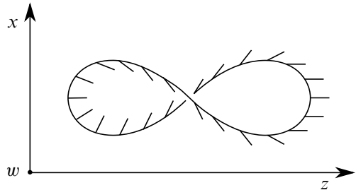
Figure 2: Cross section of a transverse torus that is C^0 -close to a transverse knot \gamma .
