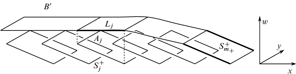
Figure 10: Parts of L , L_j and A_j .
