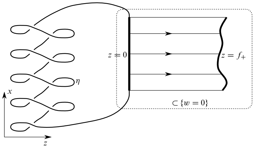
Figure 8: Front projection of the transverse curve \eta .
