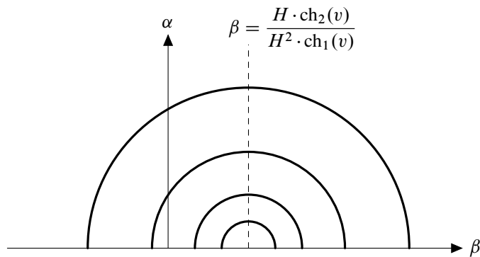
Figure 2: Walls are nested semicircles (Theorem 4.12(iii)).
