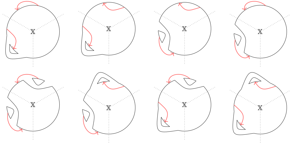
Figure 5: The off-diagonal resolution configurations in case II. The first four configurations are realized up to isotopy by expressions of the form (*1, 0*) \in \underline{\mathbb{Z}}_q^2 \times \underline{\mathbb{Z}}_r^2 and their permutations, while the last four are obtained from permutations of (*1, *1) \in \underline{\mathbb{Z}}_q^2 \times \underline{\mathbb{Z}}_r^2 .
