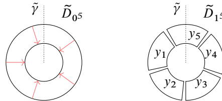
Figure 3: The \mathbb{V} \otimes \mathbb{V} \rightarrow \mathbb{W} case for p = 5 . The map downstairs is x_1, x_2 \rightarrow x , where x_1, x_2 \in Z(D_0) and x \in Z(D_1) . Let Z(\tilde{D}_{05}) = \{\tilde{x}_1, \tilde{x}_2\} , the elements over x_1 and x_2 , and let Z(\tilde{D}_{15}) = \{y_1, \dots, y_5\} , related by the action of \mathbb{Z}_5 . Then upstairs the map on fixed points is \tilde{x}_i \rightarrow (y_5 - y_1)(y_1 - y_2)(y_2 - y_3)(y_3 - y_4)y_5 = y_1 y_2 y_3 y_4 y_5 . Moreover, the element 1 \in \mathfrak{F}'_o(0^5) is sent to a term in \mathfrak{F}'_o(1^5) which is killed by projection to the summand of invariant generators, and the element \tilde{x}_1 \tilde{x}_2 is annihilated by \mathfrak{F}'_o(\phi_{05,15}^{\text{op}}) . This verifies Lemma 6.10 in this example.
