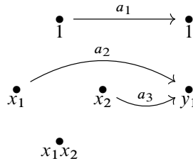
Figure 1: An example Burnside functor F: \underline{\mathbb{Z}}^1 \rightarrow \mathcal{B}_{\mathbb{Z}_2} . We visualize elements of F(1) and F(0) as dots, and regard the morphism F(\phi_{1,0}) as a collection of arrows. Here, we let F(1) = \{1, x_1, x_2, x_1x_2\} , the set of Khovanov generators associated to a resolution configuration of two circles, and F(0) = \{1, y_1\} , the set of Khovanov generators associated to a single circle. Set F(\phi_{1,0}) = \{a_1, a_2, a_3\} . Then s(a_i) is given by the tail of the arrow a_i , and t(a_i) is given by the head of the arrow a_i . This is the Khovanov–Burnside functor associated to two circles merging to a single circle. Generators at the same height have the same quantum grading.
