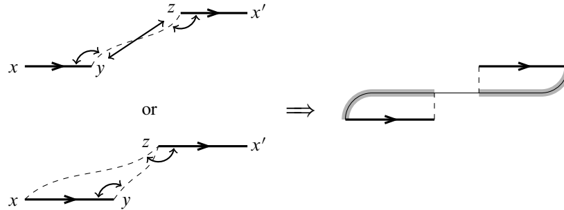
Figure 3: Schematics for Facts 2.8 and 2.9.
