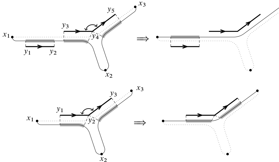
Figure 2: Schematics for Facts 2.5 and 2.6.
