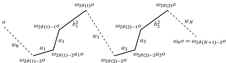
Figure 4: Words w_j , a_j and b_j that arise from a trajectory.
