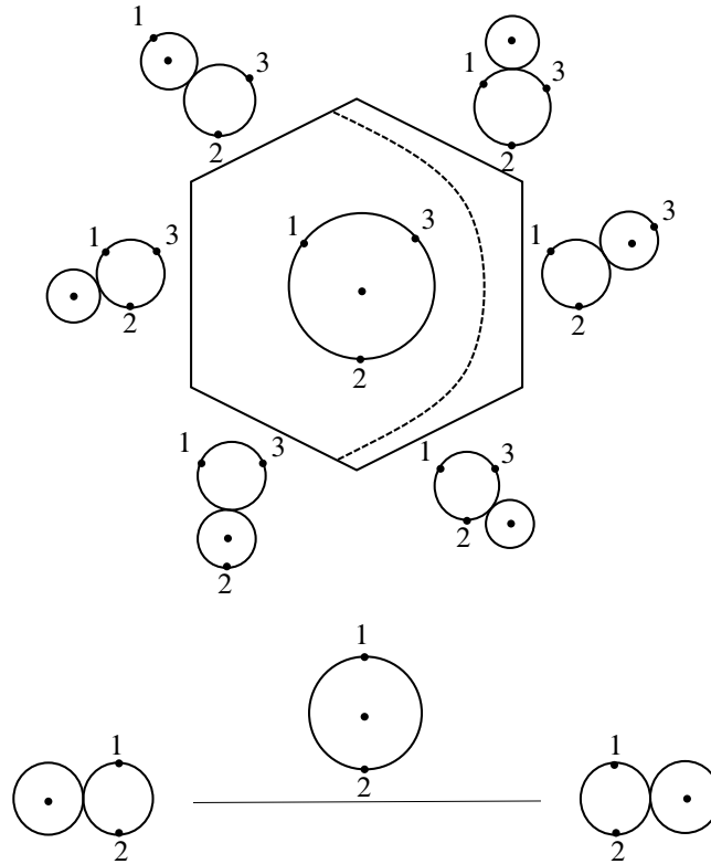
Figure 2: The hexagon represents \bar{\mathcal{M}}_{0,3,1}^{\text{main}} and the line segment represents \bar{\mathcal{M}}_{0,2,1}^{\text{main}} . The dotted line represents a typical fiber of the forgetful map. Stable marked disks are shown that represent a typical point of each space as well as a typical point of each boundary component.
