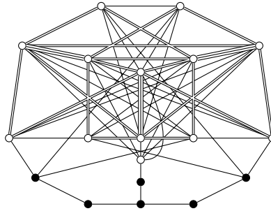
Figure 14: Dual graph of Figure 13 (1J).
