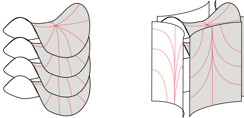
Figure 2: This is a foliation by saddles of the solid torus with four longitudinal sutures. The S^1 -direction is vertical. The limiting annular boundary leaves are added on the right. The red dotted lines denote the characteristic foliation of an approximating contact structure.
