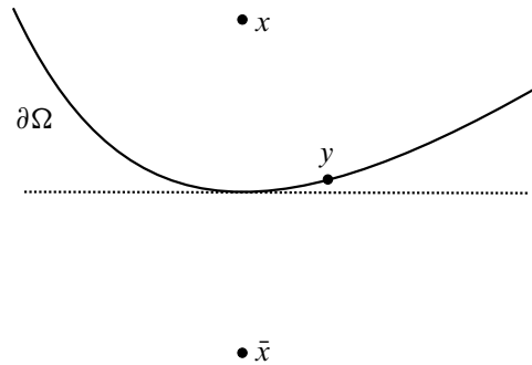
Figure 3: The dotted line is the hyperplane tangent to \partial\Omega at the origin.
