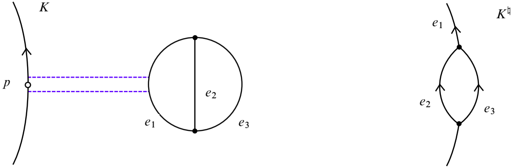
Figure 16: On the left, we take our oriented knot K and perform a connected sum with a standard theta web near the basepoint p \in K . The result is K^{\natural} on the right, and we orient the three edges of K^{\natural} as indicated.
