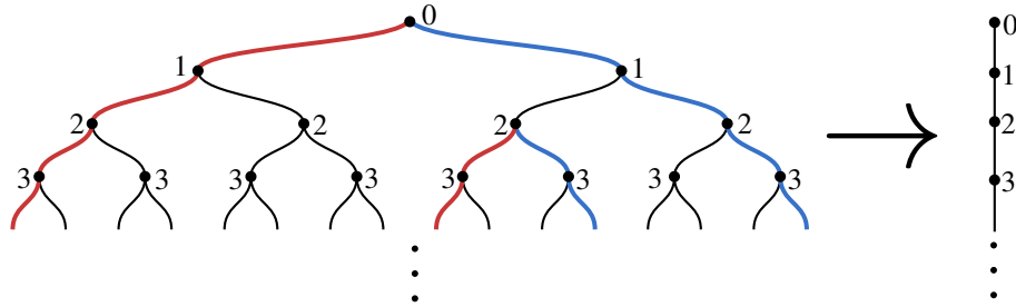
Figure 6: The red paths are of the form [v, vLLL\dots) and the blue paths are of the form [v, vRRR\dots) . Points which are equivalent with respect to the gluing are marked with the same number.
