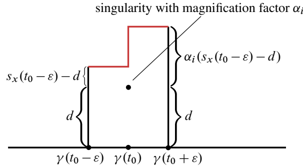
Figure 13: Constructing s_x(t) by pushing a fiber of \pi past a singularity, as seen in the image of the developing map.
