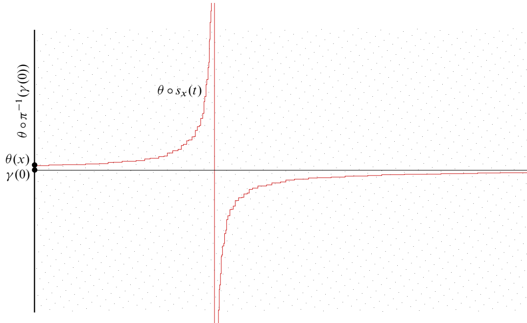
Figure 15: We continue the example from Figure 14. As before, we are drawing all objects lifted to \tilde{\Sigma}^\circ and then projected via D to \mathbb{R}^2 . The figure shows the \theta -image of a parallel section for \mathcal{J} over a curve \gamma oriented east–west. The curve \gamma is drawn as a horizontal black line in the figure. For any t , \theta \circ \pi^{-1}(\gamma(t)) would be a vertical line in the picture. The section is piecewise constant. It starts out equal to s_0 , wraps around \infty at t = t_{\max}(x) , and continues as s_1 .
