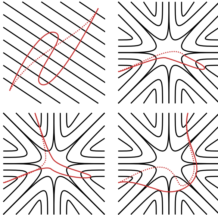
Figure 4: Various tightening moves.
