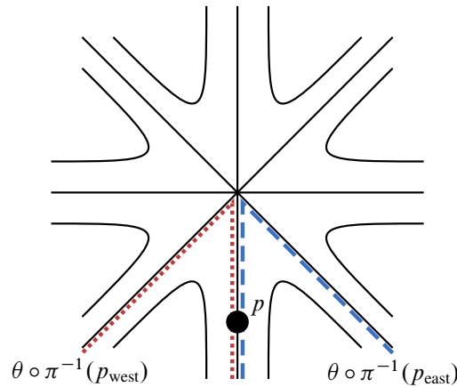
Figure 10: The unstable foliation near a singularity with k_i = 4 . The fibers over p_{\text{west}} and p_{\text{east}} are each unions of two prongs.
