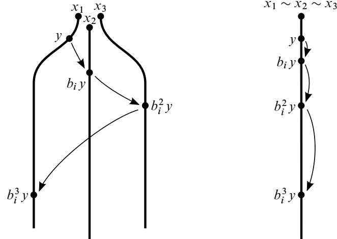
Figure 8: On the left, the action of b_i on \bigcup_{x \in O} [x, \infty) is shown for the case a_i = 3 . Here, O = \{x_1, x_2, x_3\} \subset B_i^- . The action of b_i descends to the quotient by \sim . This action on the quotient is shown on the right.
