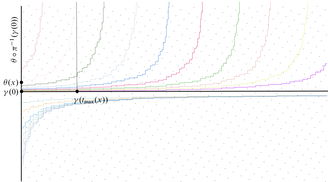
Figure 14: In this example, \Sigma^\circ = T^2 , \varphi is the monodromy of the figure-eight knot, and the surgery coefficient is (p_1; q_1) = (5, 1) . This picture shows D(\tilde{\Sigma}^\circ) \cong \mathbb{R}^2 with the 2-pronged singularities of \varphi drawn as dots. Objects in \Sigma have been lifted to \tilde{\Sigma}^\circ , and then projected to \mathbb{R}^2 via D ; for convenience in labeling the picture, we identify objects with their images under this procedure. Sections s_x(t) are shown in colors for various choices of x . These sections have been projected to \Sigma^\circ by \theta , then lifted to \tilde{\Sigma}^\circ , and finally projected to D(\tilde{\Sigma}^\circ) . Whenever x \in \pi^{-1}(\gamma(0)) satisfies x < 0 , the section s_x(t) exists for all time. When x > 0 , s_x(t) blows up in finite time.
