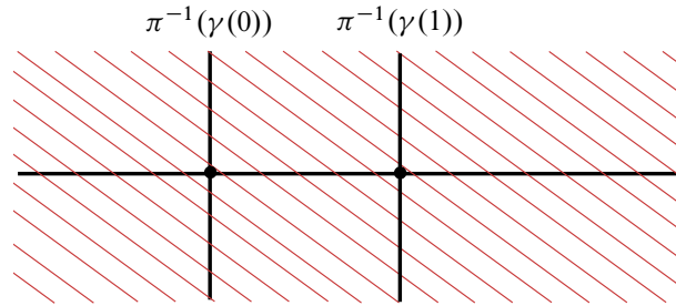
Figure 9: The total space for the bundle is shown with the fiber direction vertical. Parallel sections for the partial connection \mathcal{H} are shown in red. Each parallel section is defined only for a limited time.
