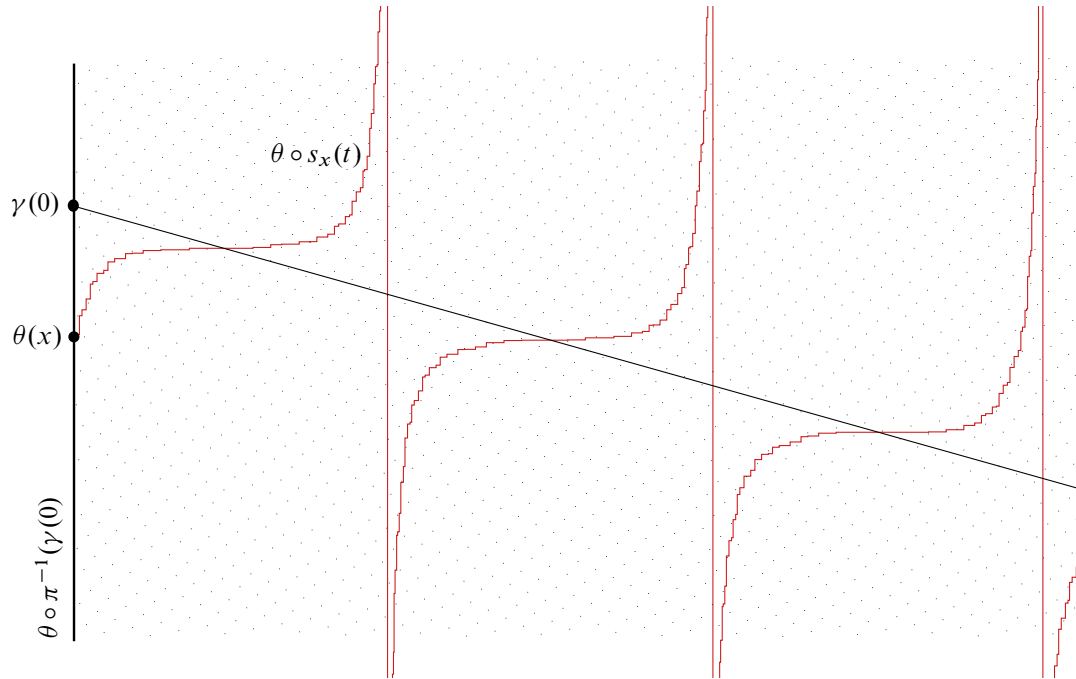
Figure 16: The \theta -image of a parallel section for \mathcal{J} over a curve \gamma of negative slope relative to the stable foliation on \Sigma^\circ . This picture is drawn with the same conventions as in Figure 15. The section s_x intersects the \infty -section infinitely many times. To see this, first homotope \gamma in \Sigma^\circ to a curve which is piecewise southward or eastward with each straight segment having length at least \varepsilon for some \varepsilon > 0 . This does not change \theta \circ s_x , since \mathcal{J} is flat. Since \gamma had negative slope and \theta \circ s_x is nondecreasing, the north-south distance between \theta \circ s_x(t) and \gamma(t) increases to C/\varepsilon in finite time, where C is the constant from Lemma 6.11. By that lemma, s_x blows up and crosses the \infty -section within the next eastward segment of \gamma . This process repeats indefinitely and produces infinitely many intersections between s_x and the \infty -section.
