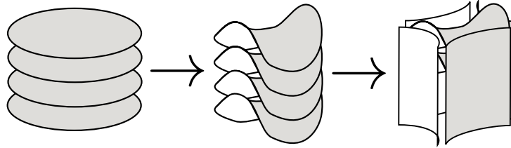
Figure 3: On the left is the standard foliation of D^2 \times S^1 , where S^1 is cut open. In the middle, we alternately comb the edges of the disks to expose their positive and negative sides. Grey shows the positive sides of the leaves, while white shows the negative sides. On the right, we show the limiting configuration which has 4 annular leaves at the boundary, which we call walls , and infinitely tall saddle-like leaves (homeomorphic to planes) on the interior. The interior saddle-like leaves accumulate on the walls. We can vary the number of legs of the saddle’s rider or the gluing of the top and bottom of the picture to get sutures of any desired nonmeridional slope.
