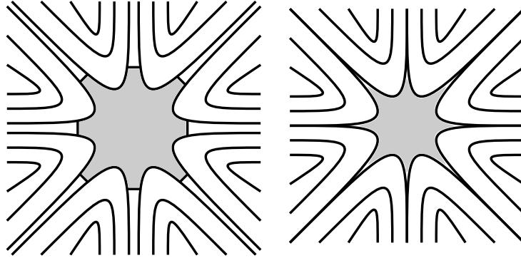
Figure 2: Blowing down \mathcal{I} . The shaded region on the left is \mathcal{G} , and the shaded region on the right is \mathcal{G}' .
