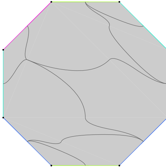
Figure 1: This figure shows a train track carrying an invariant lamination for the monodromy of the fibered, 1-cusped 3-manifold m038 . The fiber surface has genus 2 with one puncture at the vertices of the octagon. The complement of the train track is a punctured ideal hexagon. The figure was generated using Mark Bell's program flipper [2].
