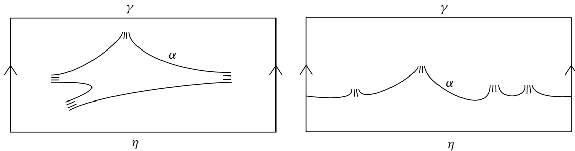
Figure 5: The annulus A is shown along with the induced foliation in a neighborhood of \alpha in two disallowed configurations. If \alpha crosses the sutures in \partial\mathcal{G} as shown, there is no way to extend the foliation to the rest of A without critical points, contradicting Roussarie–Thurston.
