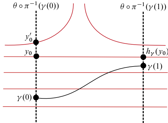
Figure 11: This is a picture in M_\varphi^\circ . The leaves of \mathcal{F}^s are shown in red. The point h_\gamma(y_0) lies on the same stable leaf as y_0 . Moreover, there exists a path from y_0 to h_\gamma(y_0) in a leaf of \mathcal{F}^s , and this path is homotopic to \gamma through paths connecting \theta \circ \pi^{-1}(\gamma(0)) to \theta \circ \pi^{-1}(\gamma(1)) . These properties uniquely specify h_\gamma(y_0) . On the other hand, h_\gamma is not defined at y'_0 .
