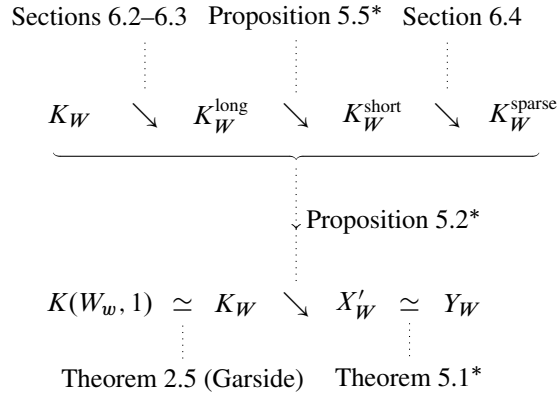
Figure 10: Relationships between the various subcomplexes of K_W and strategy of the proof of Theorem 6.1. The statements marked with an asterisk are valid for a general Coxeter group W . Note that Proposition 5.2 requires the collapses on the top row of the picture to hold for every infinite standard parabolic subgroup of W .
