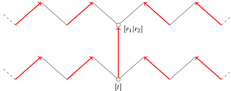
Figure 13: The matching \mathcal{M} on a fiber component of type (v) (top) and the corresponding nonexceptional component of type (iii) (bottom), as described in Sections 6.2.1, 6.2.2 and 6.2.3. The translation t is special and t = r_1 r_2 is its increasing factorization.
