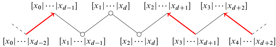
Figure 11: A matching on an infinite d -fiber component leaving the critical simplices [x_1 | \dots | x_{d-1}] , [x_1 | \dots | x_d] , and [x_2 | \dots | x_d] unmatched. More generally, one can construct a similar matching that leaves an arbitrary finite set of contiguous critical simplices unmatched, starting and ending with (d-1) -dimensional simplices. This matching is acyclic and proper.
