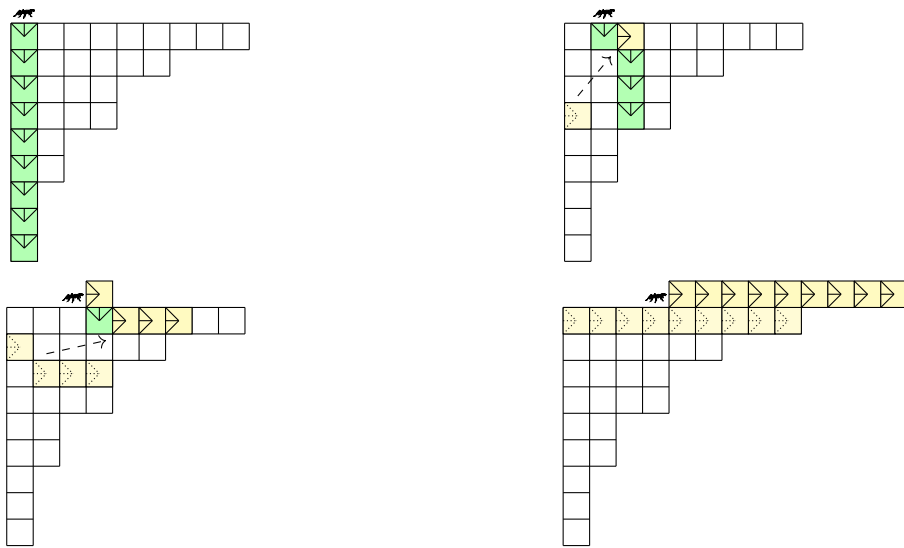
Figure 6: The first through fourth walking paths (in lexicographic order).
