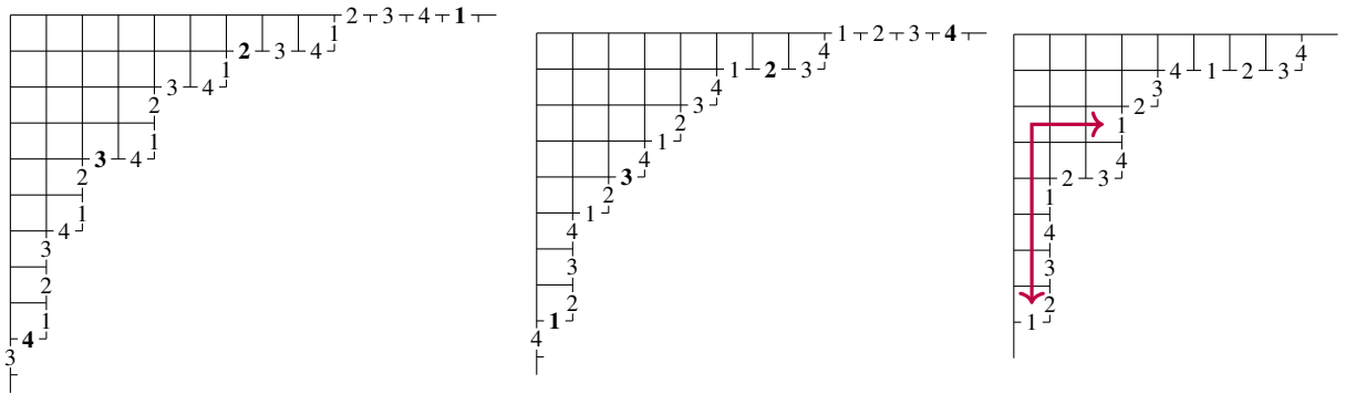
Figure 1: Left: a 4-staircase is 4-core. Center: another 4-core that is not a 4-staircase. Right: a diagram that is not a 4-core.
