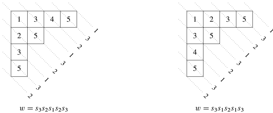
Figure 3: The two efficient fillings of this 3-staircase diagram.
