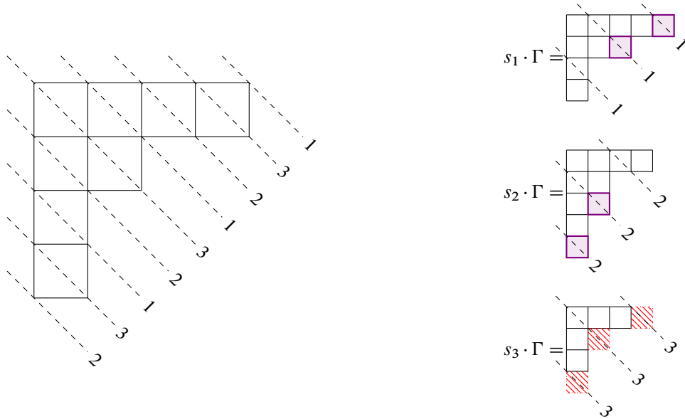
Figure 2: A 3-core diagram \Gamma (left) and the action of \tilde{S}_3 on it (right).
