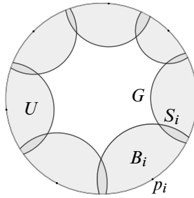
Figure 1: A framed collar U with frame G .
