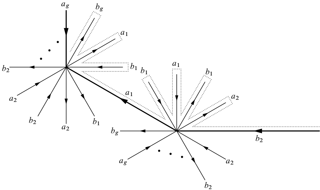
Figure 5: A piece P of \widehat{L}_w in the case when the reduced form of w contains a_g a_1^{-1} b_2^{-1} as a subword. The edges of L_w are bold. The piece is indicated by the dotted lines. This piece P has \epsilon(P) = 2 , \mathfrak{h}\epsilon(P) = 7 and \chi(P) = 1 . Note that a piece may also run along the other side of L_w .
