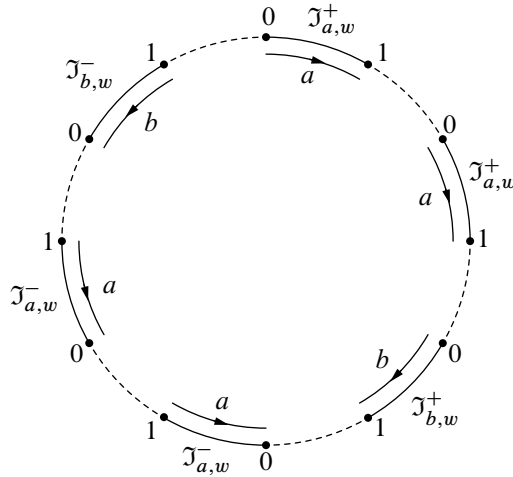
Figure 1: The w -loop for w = a^2ba^{-2}b^{-1} . The solid intervals are w -intervals and the dashed intervals are w -intermediate-intervals. We also label each interval by the set, eg \mathcal{J}_{a,w}^+ , to which they belong.
