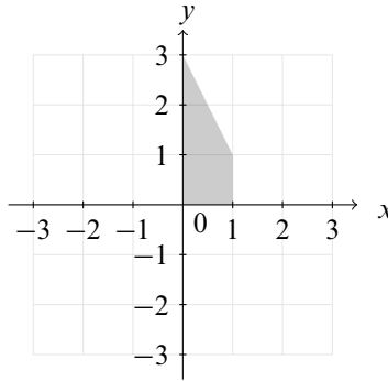
Figure 1: Okounkov body.
