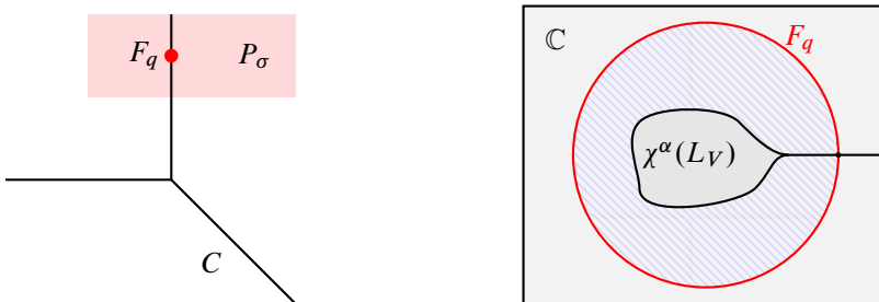
Figure 9: Monomial admissibility forces strips with \langle \partial u, \alpha \rangle > 0 to have large symplectic area. Left: condition on a tropical curve. Right: projection on \chi^\alpha : X_A \rightarrow \mathbb{C} .
