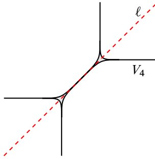
Figure 6: The projection to the base of the Lagrangian torus fibration of a tropical Lagrangian. The holomorphic cylinder above the red dashed line cleanly intersects the tropical Lagrangian.
