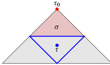
Figure 6: Illustration for G = \text{PSL}(4, \mathbb{R}) of a connected component \sigma of \mathbb{S}\mathfrak{a}^+ \setminus \bigcup_{w \in W} (w \cdot \tau)^\perp in an affine chart.
