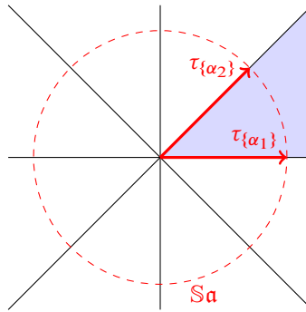
Figure 3: The model restricted Cartan algebra \mathfrak{a} and its Weyl chamber \mathfrak{a}^+ for \text{PSp}(4, \mathbb{R}) .
