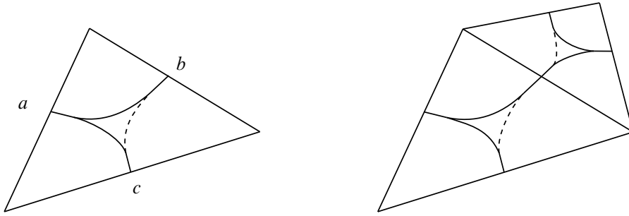
Figure 2: The 1-complex and the train track dual to a triangulation. The train track is obtained by removing the dashed edges from the 1-complex. Left: the dual 1-complex and dual train track in a triangle. Right: joining the dual 1-complexes and train tracks.
