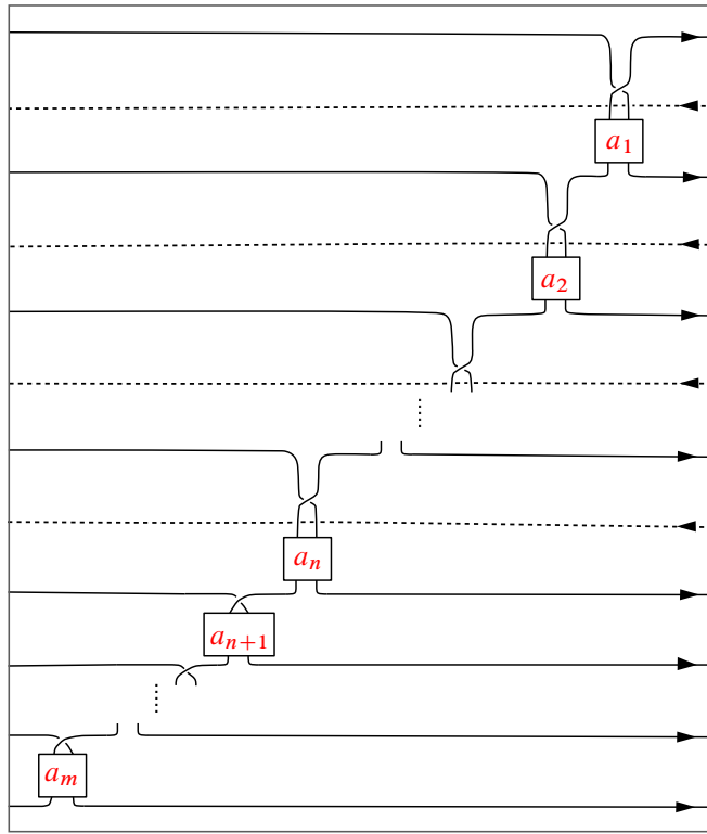
Figure 8: The pattern P' (omit horizontal dotted lines) and P'' (include horizontal dotted lines).
