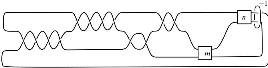
Figure 6: A Kirby diagram for a cobordism (W, S_{m,n}): (S^3, K_{m,n}) \rightarrow (S^3, K_{m,n+1}) . The cobordism is obtained by attaching the (-1) -framed 2-handle to (S^3, K_{m,n}) .
