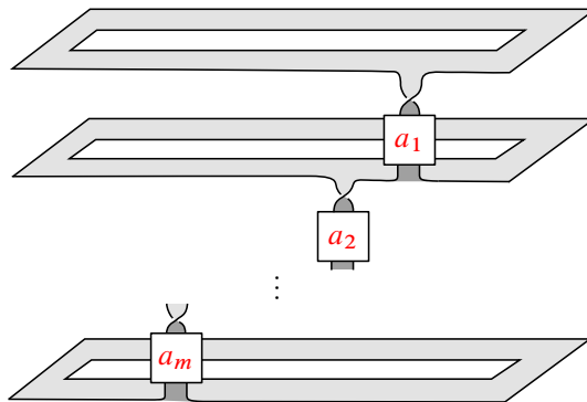
Figure 9: The surface \bar{S} .
