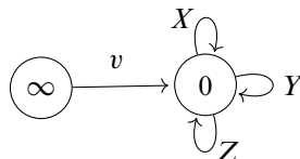
Figure 1: Quiver for the noncommutative Hilbert scheme.
