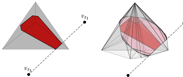
Figure 12: Left: the hexagon \Sigma_T , embedded in the tetrahedron F_D . The subset \Sigma_{t_1, t_3} is an edge of the hexagon contained in the bottom face F_{D \cup E} of F_D . Right: the convex subset P_{\min} embedded in the polytope P .
