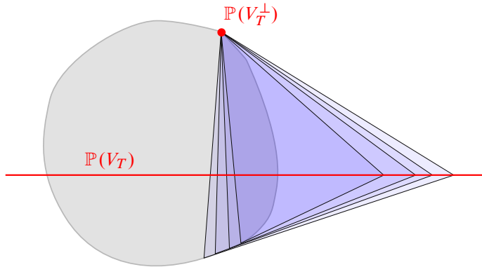
Figure 3: A sequence of nested half-cones over walls in an itinerary W_1, \dots, W_n where \overline{W}_1 \cap \overline{W}_n \neq \emptyset . Lemmas 7.3 and 7.4 show that if the element traversed by this itinerary has large singular value gaps, then its unstable subspace lies in Hc_+(W_k) for some large k , and is far from \overline{W}_1 \cap \overline{W}_n . In particular, the subspace is far from the complement of Hc_+(W_1) .
