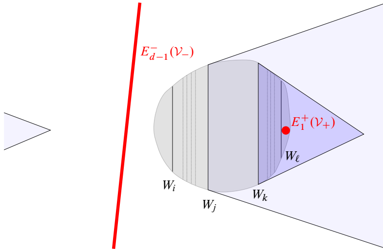
Figure 4: Illustration for the proof of Lemma 8.15. Since the half-cones over W_j, W_k strongly nest, the subspaces E_1^+(\mathcal{V}_+) and E_{d-1}^-(\mathcal{V}_-) are uniformly transverse.
