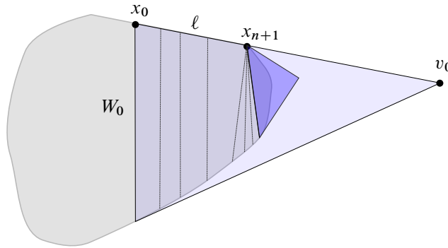
Figure 2: Illustration for the proof of Lemma 5.15. The walls separating W_0 from W_{n+1} all intersect either the interior of \ell \cup R_0\ell , or the endpoint x_{n+1} .
