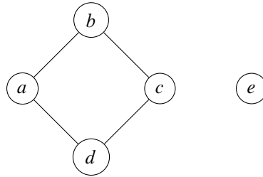
Figure 6: The nerve of the right-angled Coxeter group C in Proposition A.1 (recall that there is an edge between two vertices in the nerve precisely when the corresponding generators commute).
