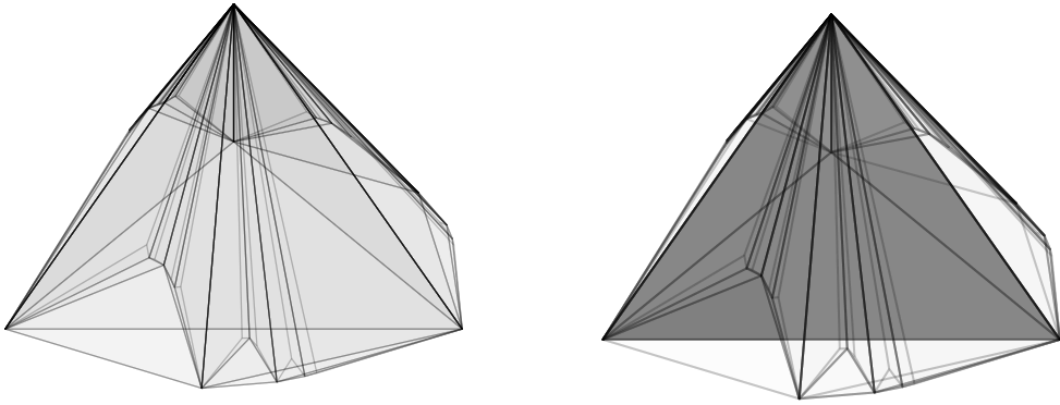
Figure 10: The convex polytope P (left and right). On the right, the tetrahedral fundamental domain F_D has also been highlighted. The reflections t_1, t_2, and t_3 in the three faces of F_D meeting at the topmost vertex preserve the polytope P , while the reflection e in the bottom face F_{D \cup E} does not.
