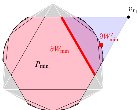
Figure 13: The boundary of the half-cone over W_{\min} intersects the boundary of the wall W'_{\min} .
