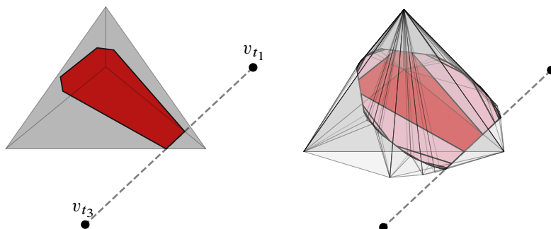
Figure 12: Left: the hexagon \Sigma_T , embedded in the tetrahedron F_D . The subset \Sigma_{t_1,t_3} is an edge of the hexagon contained in the bottom face F_{D \cup E} of F_D . Right: the convex subset P_{\min} embedded in the polytope P .
