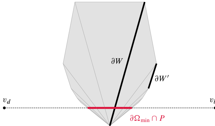
Figure 8: The boundary of the minimal reflection domain \Omega_{\min} does not contain a segment joining W with W' . See Theorem A.7 below for a construction of \Omega_{\min} .
