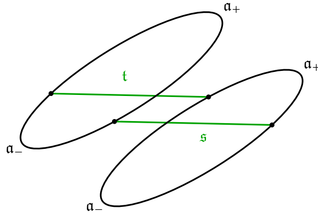
Figure 11: Proof sketch of Proposition 4.3: joining \gamma_0 and \gamma_1 via segments \mathfrak{s} and \mathfrak{t} .
