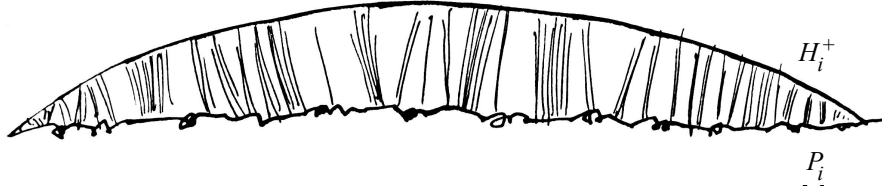
Figure 3: A visualization of the map F_i^\eta , flowing normally from P_i^\eta till H_i^+ . Lemma 2.5 below shows that these lines indeed do not meet for i large enough.
