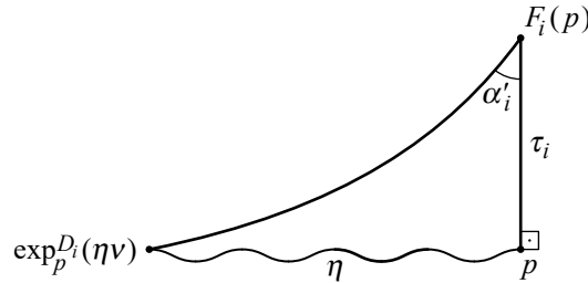
Figure 7: The angle \alpha'_i is defined in a similar way to \alpha_i , except that it is opposite to an intrinsic geodesic of D_i of length \eta , rather than a geodesic of \mathbf{H}^3 .
