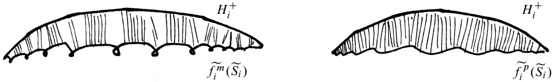
Figure 1: Visual outline of the proof of Theorem 2.1. We will flow the universal covers \tilde{f}_i^m(\tilde{S}_i) and \tilde{f}_i^p(\tilde{S}_i) of the asymptotically Fuchsian minimal and pleated surfaces normally till they hit a component H_i^+ of the boundary of the convex core. We will argue this process has a uniformly small area distortion (away from the pleating lamination, in the pleated case).
