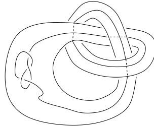
Figure 11: A swallow-follow torus
