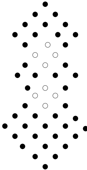
Figure 5: A cancellation principle
