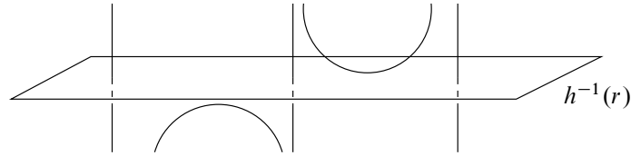
Figure 7: After the isotopy
