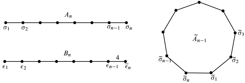
Figure 1: Coxeter graph of type A_n , B_n ( n \geq 2 ) and \tilde{A}_{n-1} ( n \geq 3 ). Labels equal to 3, as usual, are not shown. Moreover, to fix notation, every vertex is labelled with the corresponding generator in the Artin group.
