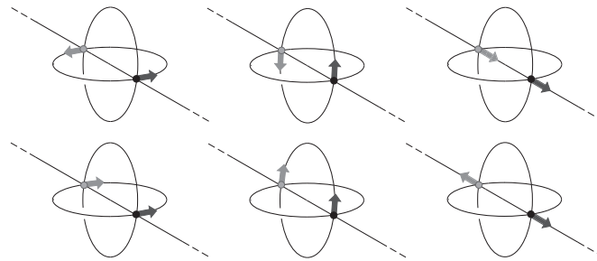
Figure 14: 3 spacelike pencils (above) and 3 timelike pencils (below)
