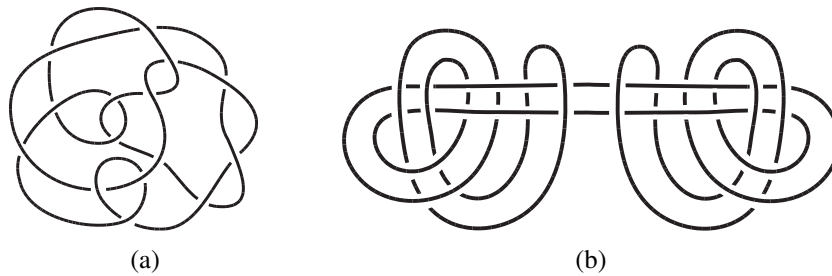
Figure 9: (a) Ochiai's unknot (b) Freedman's unknot
