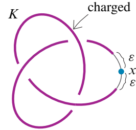
Figure 4: The subarc \{y \in K \mid d_K(x, y) \geq \epsilon\}
