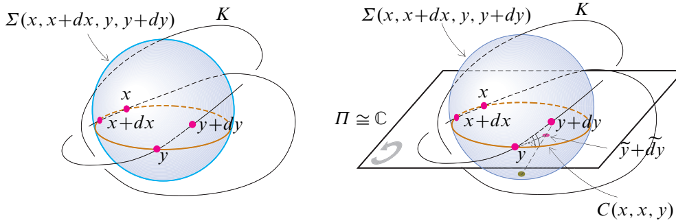
Figure 12: A stereographic projection
