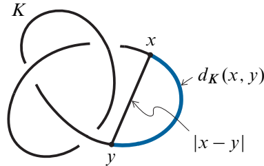
Figure 3: The arc-length and the chord length
