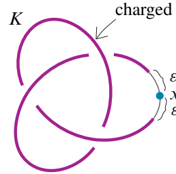
Figure 4: The subarc \{y \in K \mid d_K(x, y) \geq \varepsilon\}
