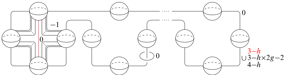
Figure 2: Handle diagram of a genus- g Torelli BLF
