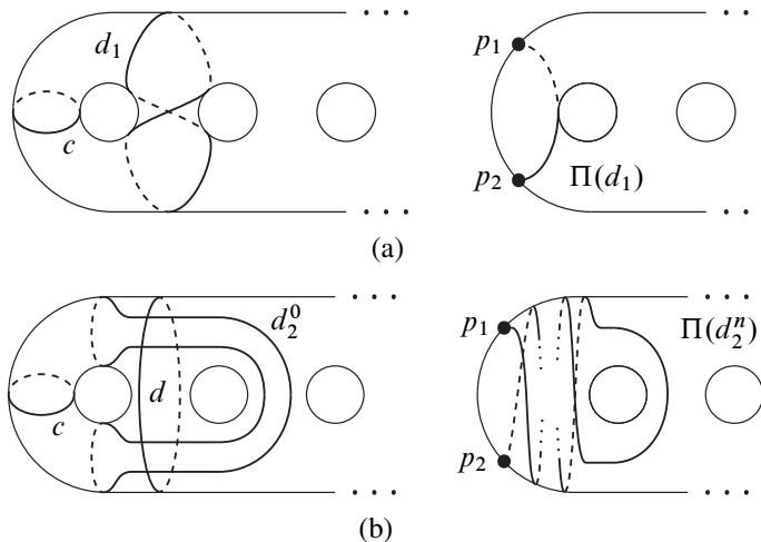
Figure 3: Separating curves and corresponding paths
