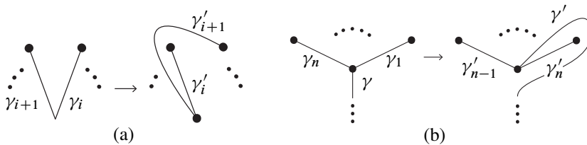
Figure 1: Modifications of Hurwitz path systems
