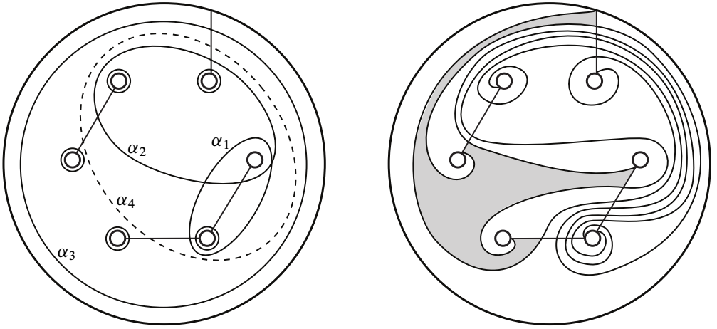
Figure 20: \begin{pmatrix} a_1 & b_1 \\ a_2 & b_2 \\ a_3 & b_3 \end{pmatrix} = \begin{pmatrix} 1 & 2 \\ 1 & 3 \\ 3 & 1 \end{pmatrix}
