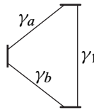
Figure 5: \{\gamma_1, \gamma_a\} \rightsquigarrow \{\gamma_1, \gamma_b\} is an arc slide
