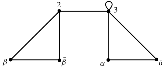
Figure 1. G(18) in \mathbb{Z}[\sqrt{-5}] .
