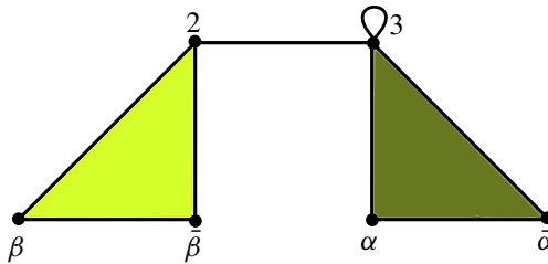
Figure 4. S(18) in \mathbb{Z}[\sqrt{-5}] .
