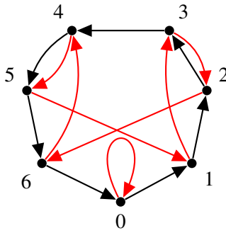
Figure 1. The graph D_7 , used to determine divisibility by 7.
