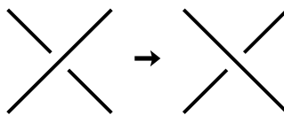
Figure 2. Crossing change.
