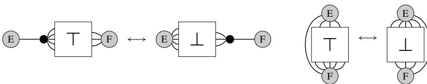
Figure 9. Graph equivalents of a flype.
