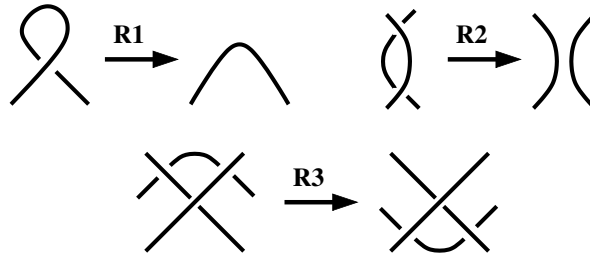
Figure 1. Reidemeister moves.
