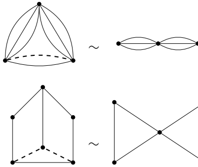
Figure 16. Top: 8_5 \geq 3_1 \# 3_1 . Bottom: 8_{16} \geq 3_1 \# 3_1 .
