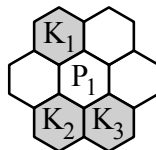
Figure 9. The special case for k = 2 and k = 3 .
