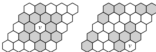
Figure 2. Some examples of \mathcal{R}(v) shaded on a 5 \times 5 board.
