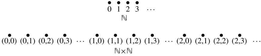
Figure 1. The set \mathbb{N} of natural numbers relative to the usual order (above) and the set \mathbb{N} \times \mathbb{N} with the dictionary order (below).
