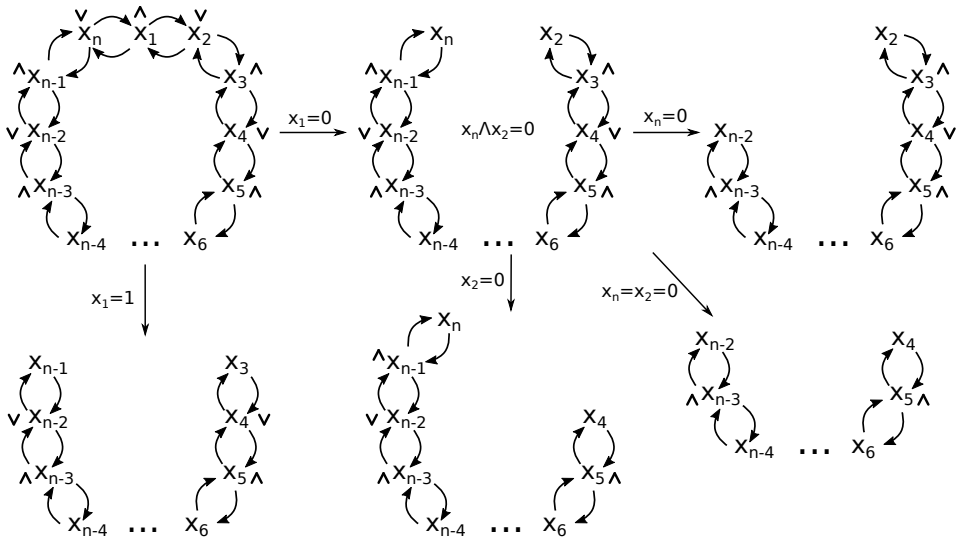
Figure 3. Idea behind the proof of Proposition 3.1.2 (logical operators are included for clarity). Considering the case x_1 = 1 yields a system of equations that corresponds to a smaller AND-OR network. Considering the case x_1 = 0 yields a system of equations that does not correspond to an AND-OR network (due to the equation x_n \wedge x_2 = 0 ). However, the subcases x_n = 0 and x_2 = 0 yield systems of equations that do correspond to smaller AND-OR networks. These two systems have overlapping solutions, so we must also take into consideration the common case x_n = x_2 = 0 when counting the number of fixed points.
