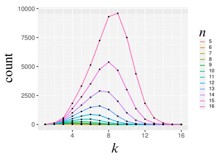
Number of k -term 4-pseudo progressions in \{1, 2, \dots, n\} .
