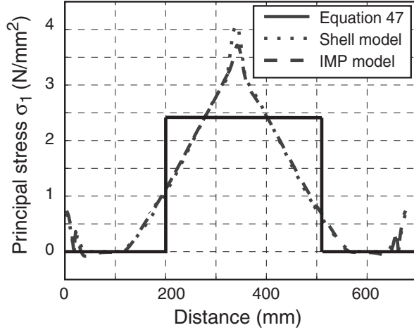
Figure 19. Distribution of midsurface principal stress along a diagonal, for T_1/T_2 = 4 .
