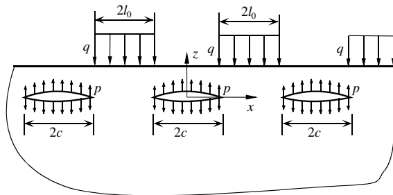
Figure 13. Crack model for cutting a periodic array of straight grooves.
