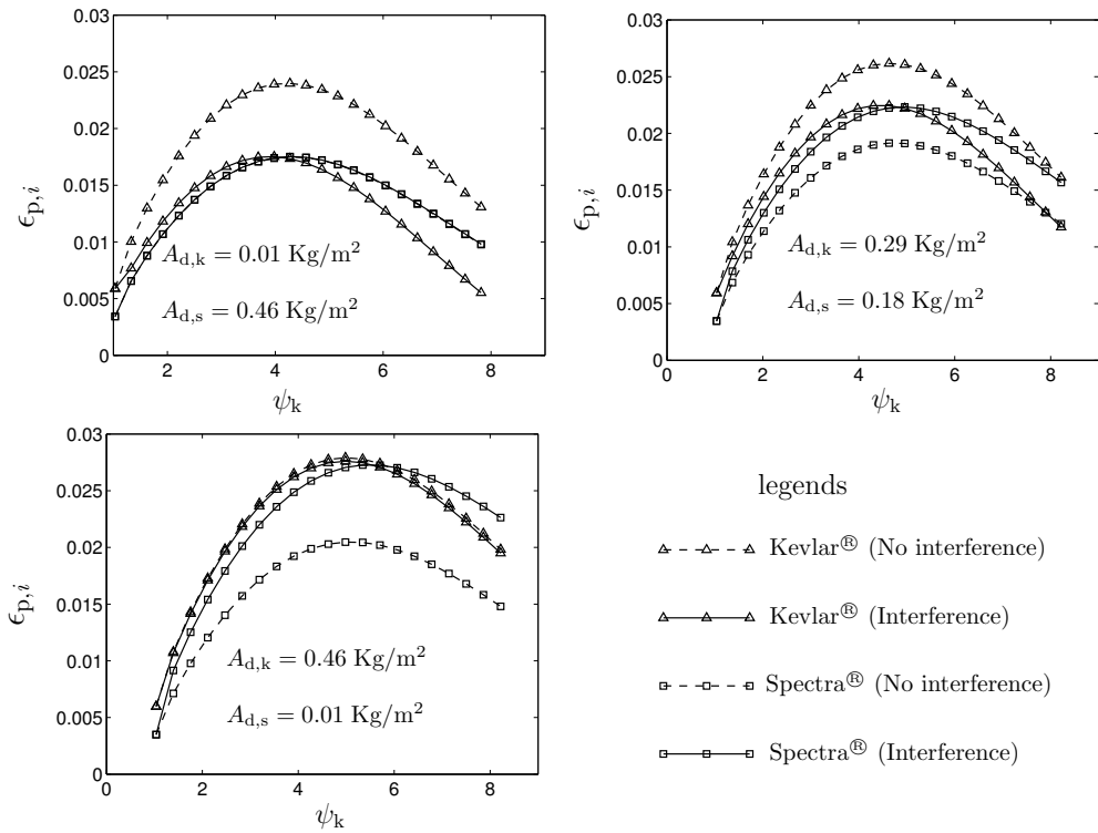
Figure 3. Strains in the layers around the projectile tip versus normalized cone wavefront for both interfering and noninterfering arrangements under impact velocity V_p = 140 \text{ m/s} . The x-axis coordinate, \psi_k , is the wavefront position of the Kevlar layer when in the noninterfering arrangement. In the first figure the strains for interfering and noninterfering arrangement coincide for Spectra layer.
