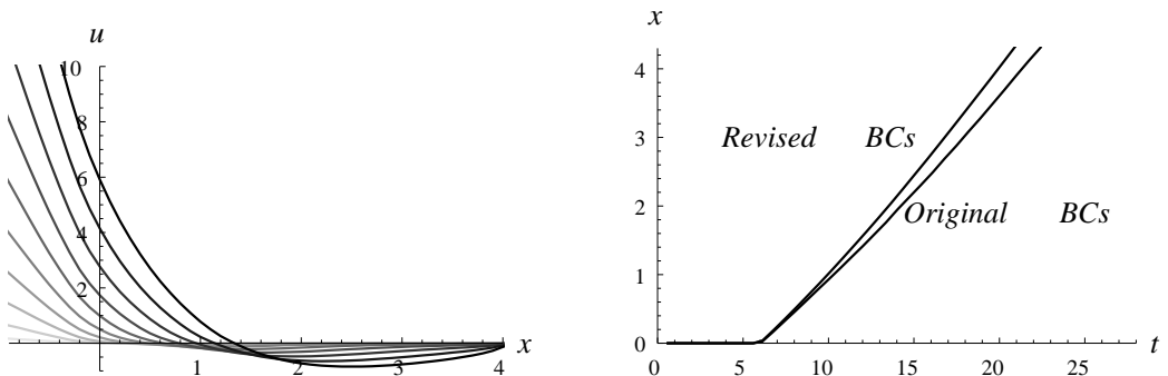
Figure 4. Example with b = 2 , showing negative displacements from integral equation calculations under the assumption that the unloaded crack faces and the region to the right of the cohesive zone will be stress-free. The graph on the left shows the displacement profiles at times t = 1, 2, \dots, 10 (in dimensionless units), where the crack tip begins accelerating at t \approx 6.1 . While these negative displacements are very small compared to those in the loading interval, they do have a significant effect in preventing the crack faces from properly opening and so significantly impact transient crack tip calculations, as shown in the graph (t) on the right of the crack tip position x = \ell(t) .
