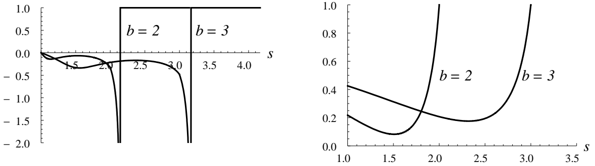
Figure 1. Graph of G_1(s) - H(c - s)B\sqrt{(c - a)/(c - s)} on the left and of G_2(s) on the right for a = 1 , b = 2.0, 3.0 , and c \approx 2.14, 3.17 , respectively. The function G_1(s) - H(c - s)B\sqrt{(c - a)/(c - s)} involves a square root singularity and sign switch at s = c = 1/c_R , while G_2(s) is always positive.
