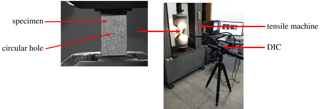
Figure 4. Experimental equipment.
