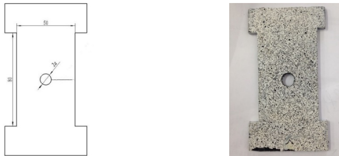
Figure 3. Experimental specimen. Left: specimen size (mm). Right: painted specimen.
