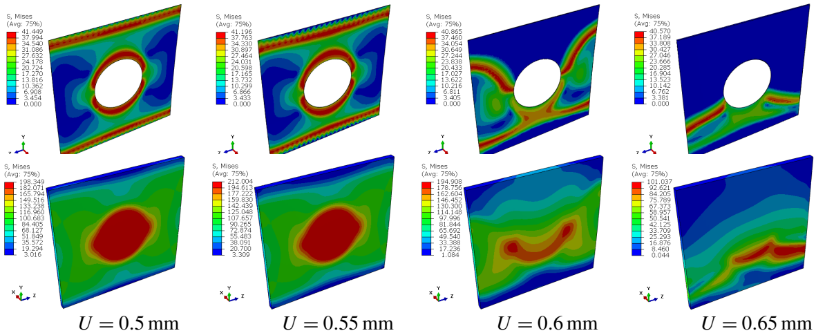
Figure 16. Von Mises stresses in the adhesive Araldite 420 and the composite patch for different imposed displacements U .
