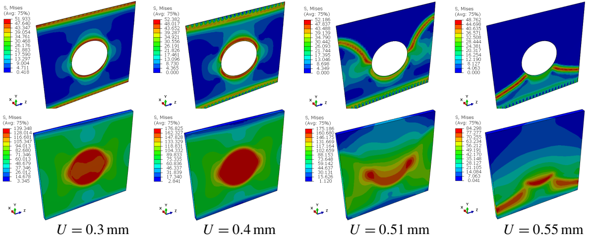
Figure 17. Maximal von Mises stresses in the adhesive AV138 and the composite patch for different imposed displacements U .
