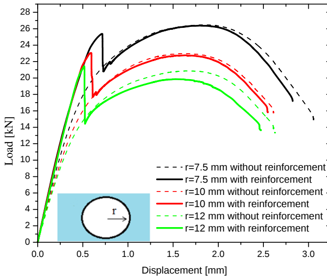
Figure 8. Load-displacement curves for different dimensions (radius) of circular notch (plate repaired with Araldite AV138).
