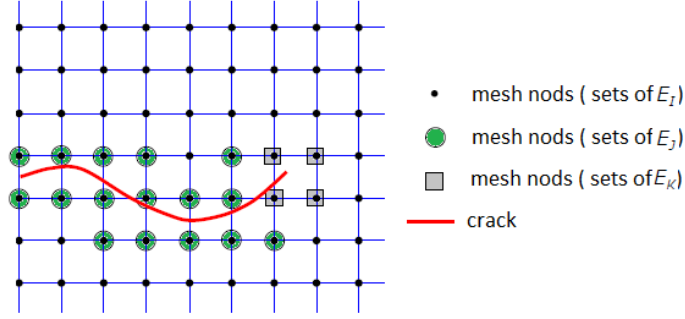
Figure 1. Description of the E_1 , E_J and E_K sets of the displacement field approximation enriched finite element.
