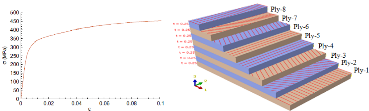
Figure 5. Left: tensile stress-strain curve of aluminum plate. Right: the stacking sequence of composite used.
