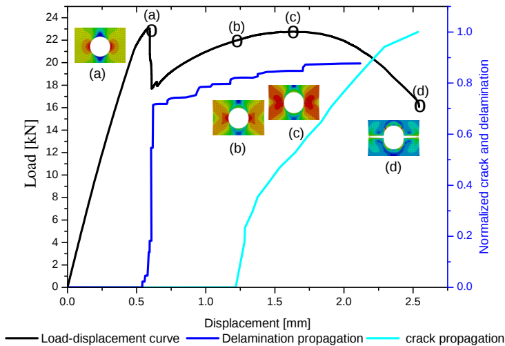
Figure 14. Force-displacement curve, the normalized crack length and debonding area for the case with circular notch of r = a = b = 10 mm with cohesive AV138; (a) start of delaminating patch, (b) start of crack propagation in Aluminium plate, (c) total damage of aluminum plate, (d) failure load.
