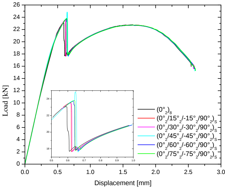
Figure 11. Failure load-displacement curves for different stacking sequences of carbon-epoxy laminate.
