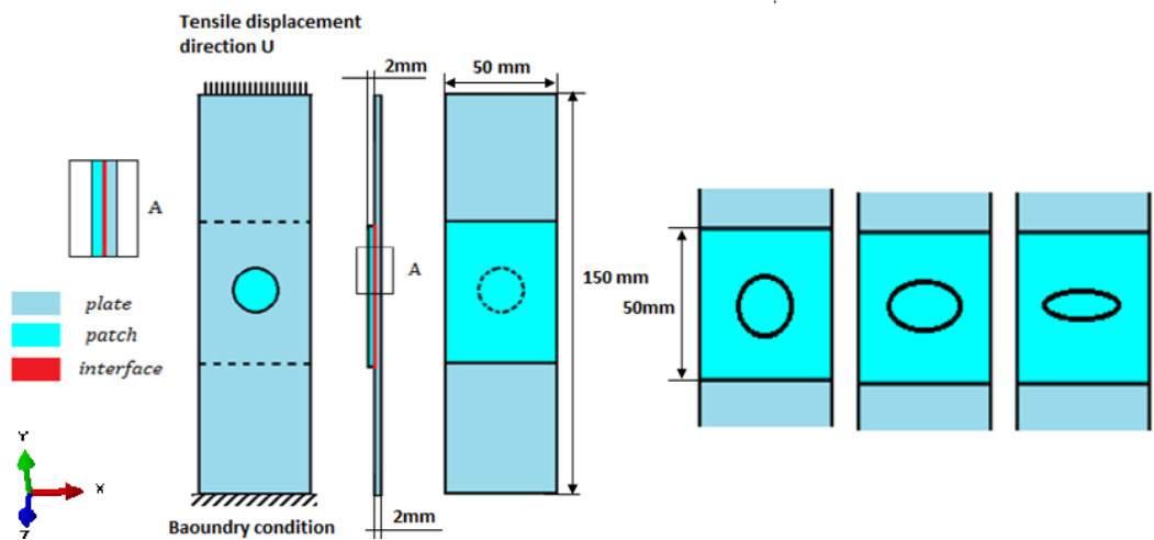
Figure 4. Geometric model of the bonded system.
