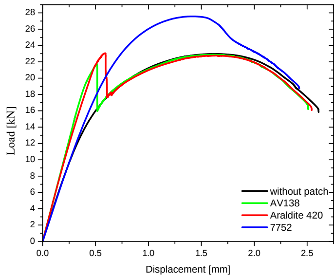
Figure 12. Failure load-displacement curves for different adhesives used.
