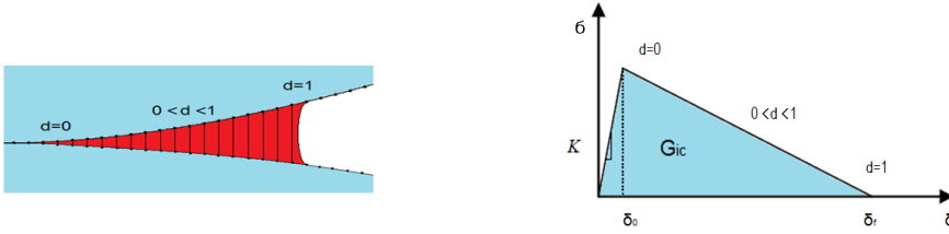
Figure 2. Linear softening law for mixed-mode cohesive damage models.
