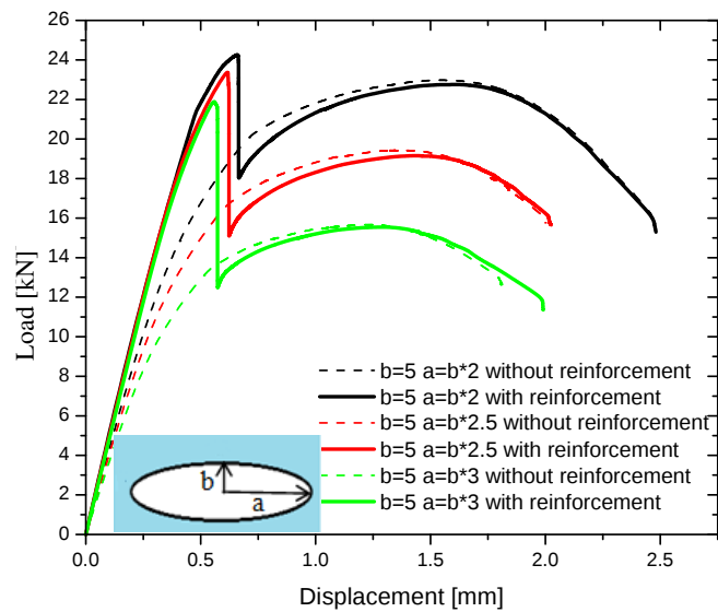
Figure 10. Load-displacement curves for different dimensions of an elliptical notch (plate repaired with Araldite AV138).
