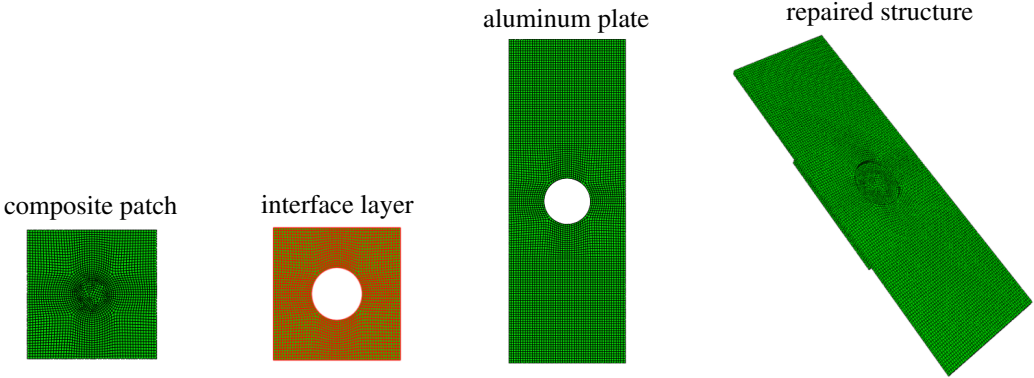
Figure 7. Details of the mesh of each region.
