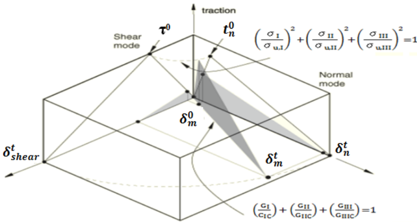
Figure 3. A traction-separation law for modeling the interface material degradation.
