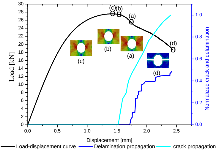
Figure 15. Force-displacement curve, the normalized crack length and debonding area for the case with circular notch of r = a = b = 10 mm with cohesive 7752; (a) start of delaminating patch, (b) start of crack propagation in aluminum plate, (c) failure load, (d) total damage of aluminum plate.
