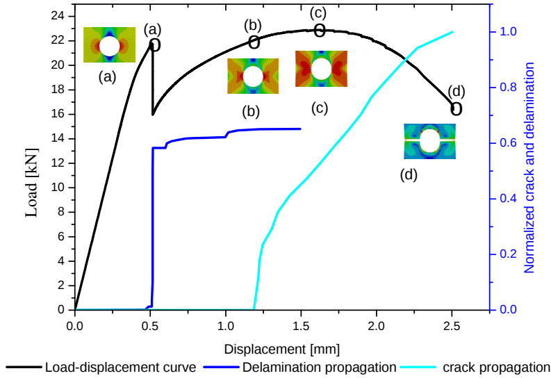
Figure 13. Force-displacement curve, the normalized crack length and debonding area for the case with circular notch of r = a = b = 10 mm with cohesive Araldite 420; (a) start of delaminating patch, (b) start of crack propagation in plate, (c) failure load, (d) total damage of aluminum plate.
