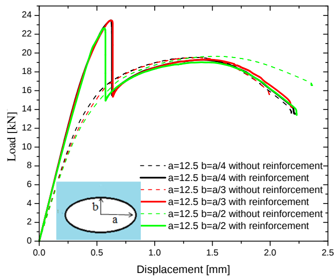
Figure 9. Load-displacement curves for different dimensions of elliptical notch (plate repaired with Araldite AV138).
