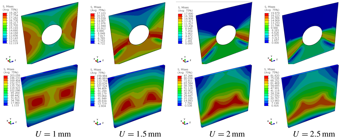
Figure 18. Maximal von Mises stresses in the adhesive 7752 and the composite patch for different imposed displacements U .
