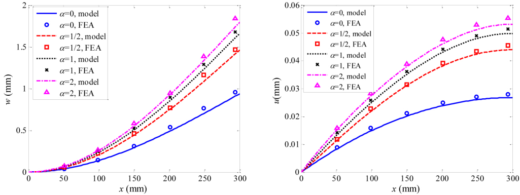
Figure 15. Comparison of vertical deflection and relative slip along the beam length for different pressure distribution laws between theoretical predictions and FEA under normal load F=160\text{N} .
