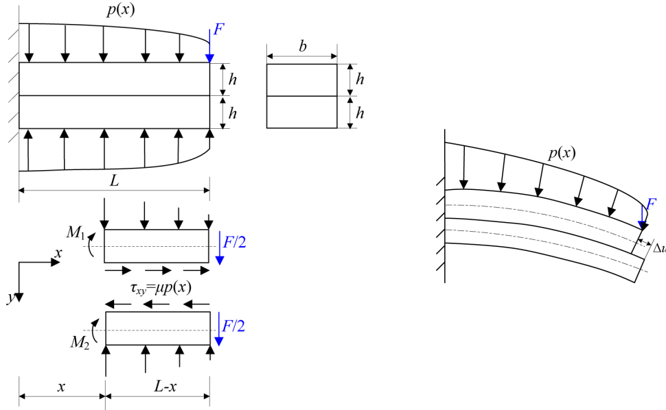
Figure 2. Left: model for examining the relative slip motion at the joint interface and the free-body diagram of the beams. Right: relative motion at the frictional interface under the vertical load, with u the relative displacement at the joint interface.
