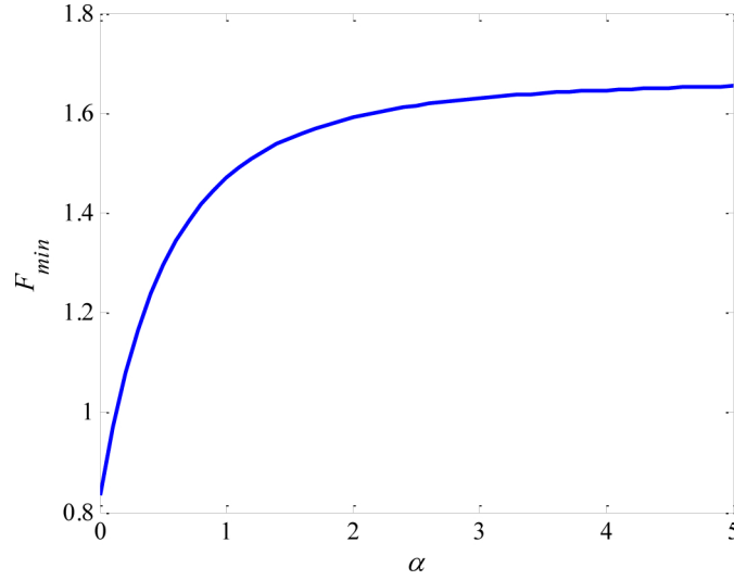
Figure 7. Variation of the minimum nondimensional normal load for relative slipping occurring as a function of pressure distribution law.
