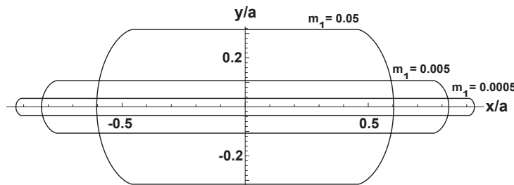
Figure 1. Variation of slot aspect ratio and shape with elliptic integral parameter.
