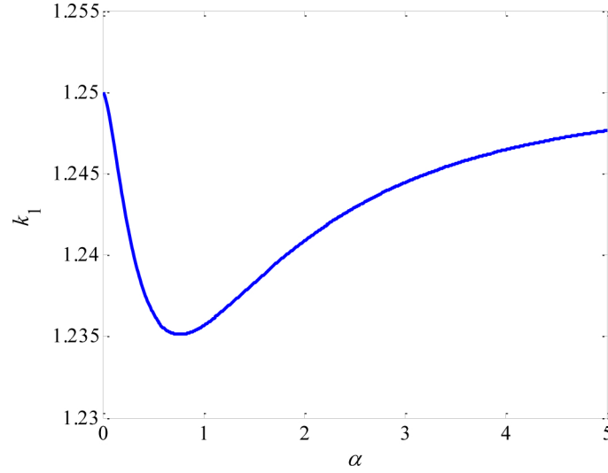
Figure 9. Variation of the slope for force-deflection relationship in the unloading process.
