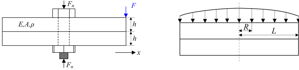
Figure 1. Left: schematic diagram of a press-fit joint under a vertical force at the free end. Right: pressure distribution along the interface.
