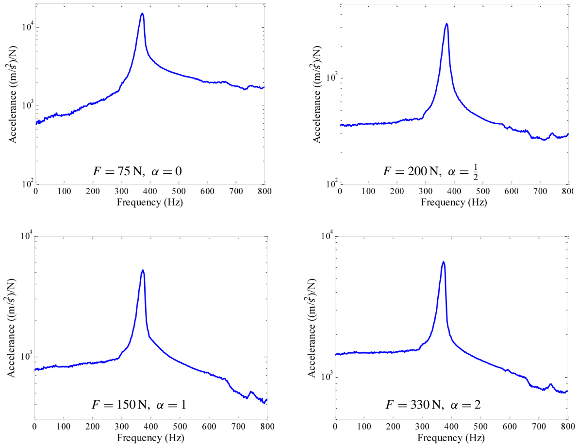
Figure 16. Frequency response function of the system for different amplitudes of impulse excitation and different pressure distribution laws.
