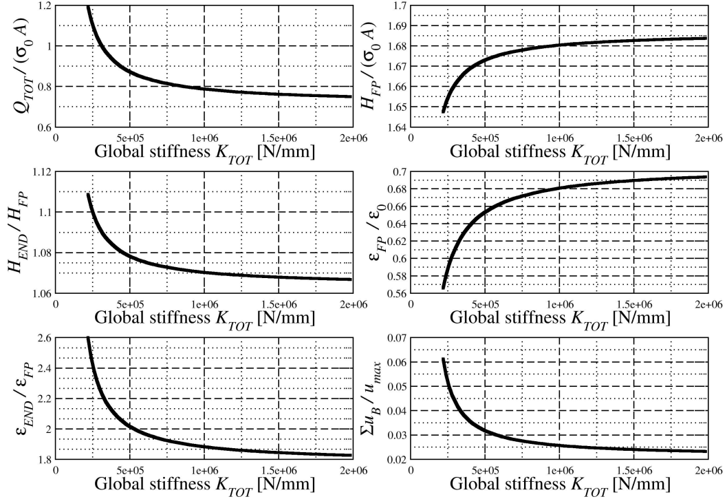
Figure 8. Reduced-scale BRB. Dependence of various mechanical quantities on the restrainer global elastic stiffness K_{TOT} . Results computed adopting \xi = 3 . Other symbols as explained in the text.
