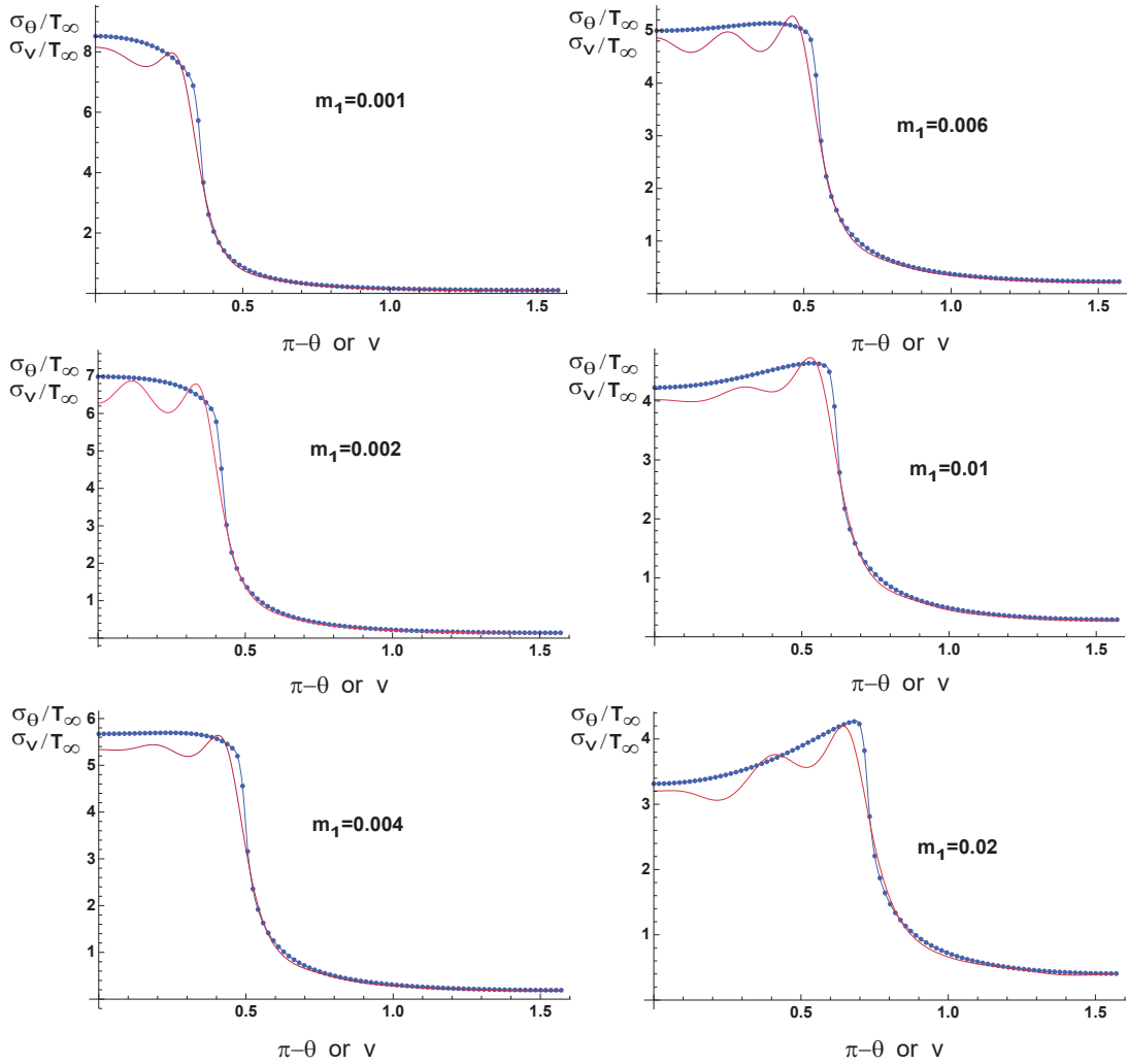
Figure 3. Stress distribution along slot surface under biaxial loading for various slot aspect ratios (3).
