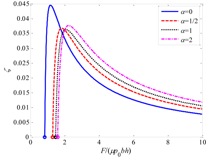
Figure 10. Plots of the relationship between damping ratio and nondimensional normal load for different pressure distribution laws. The symbol \bigcirc denotes the minimum force values inducing relative slip.
