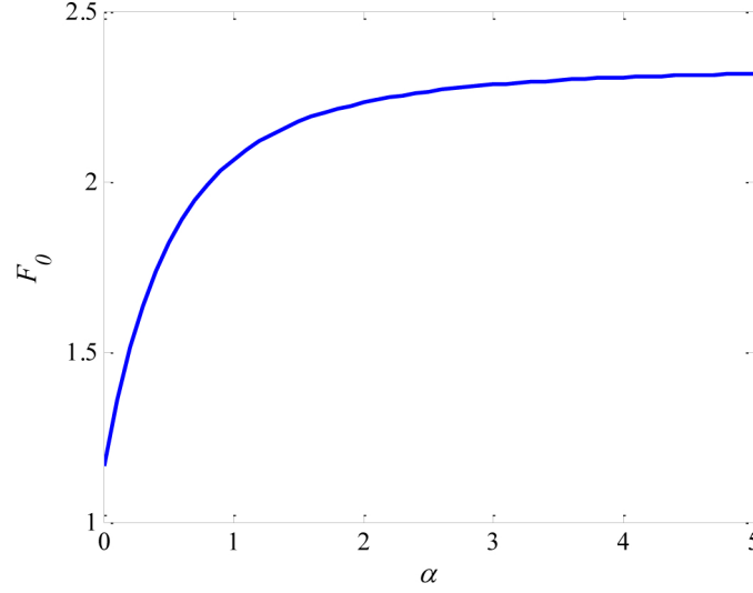
Figure 11. Plot of the variation of the normal load at which the peak damping ratio occurring with the pressure distribution law.
