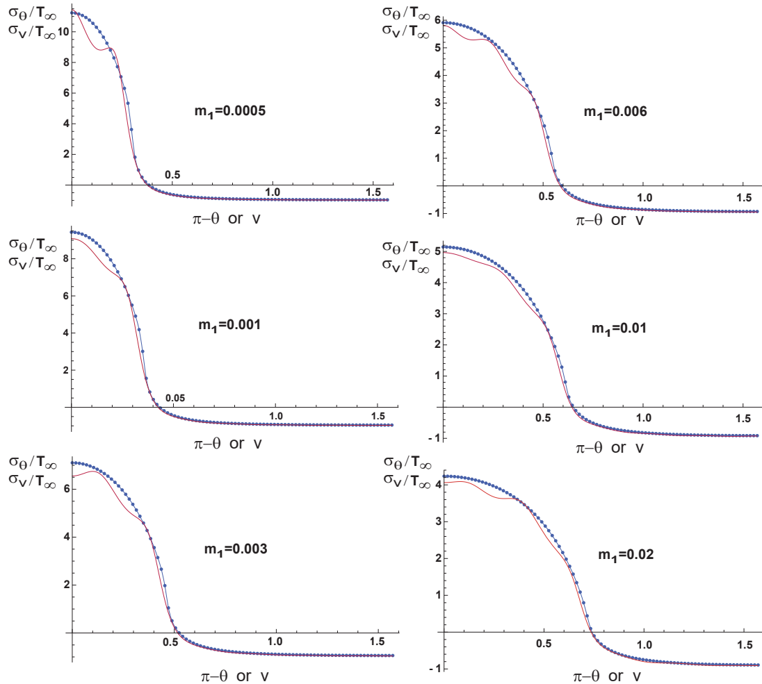
Figure 2. Stress distribution along slot surface under uniaxial loading for various slot aspect ratios (3).
