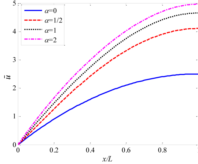
Figure 5. Nondimensional relative slip along the beam length for different pressure distribution laws. The nondimensional normal load \bar{F} = 3 .
