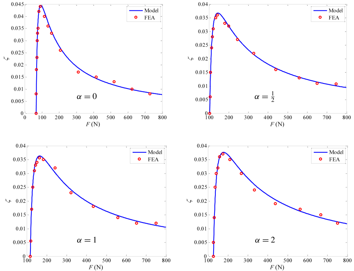
Figure 17. Comparison of damping ratio versus normal load between model predictions and FEA results for different pressure distribution laws.
