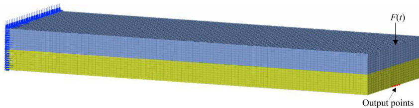
Figure 14. Finite element mesh for the layered cantilever beam model.
