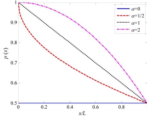
Figure 3. Pressure distributions along the interface for different laws with p_0 = 1 .
