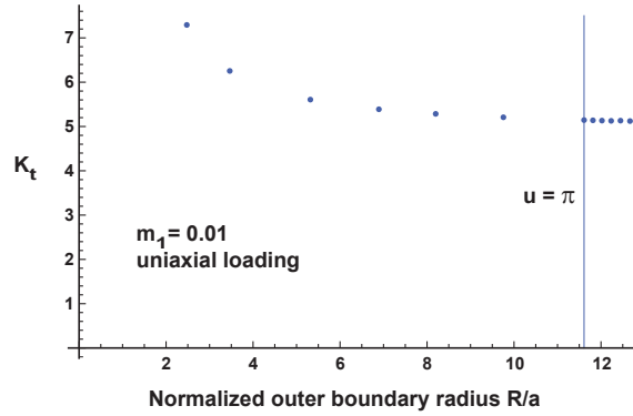
Figure 8. Convergence of numerical solution for stress concentration factor as a function of outer boundary radius.
