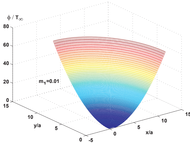
Figure 7. Airy stress function \phi for biaxial loading.
