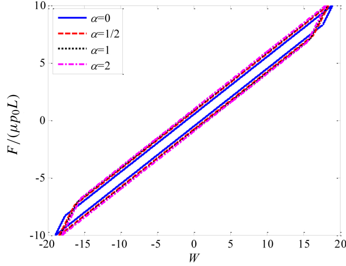
Figure 8. Effect of pressure distribution laws on the hysteresis loop.
