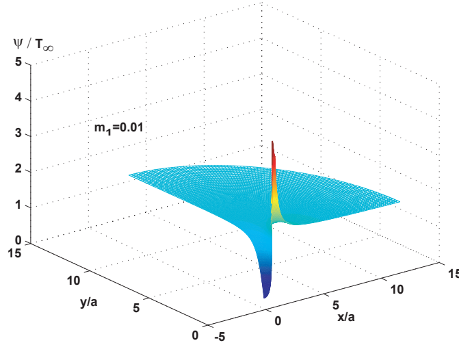
Figure 5. Sum of in-plane normal stresses \psi for biaxial loading.
