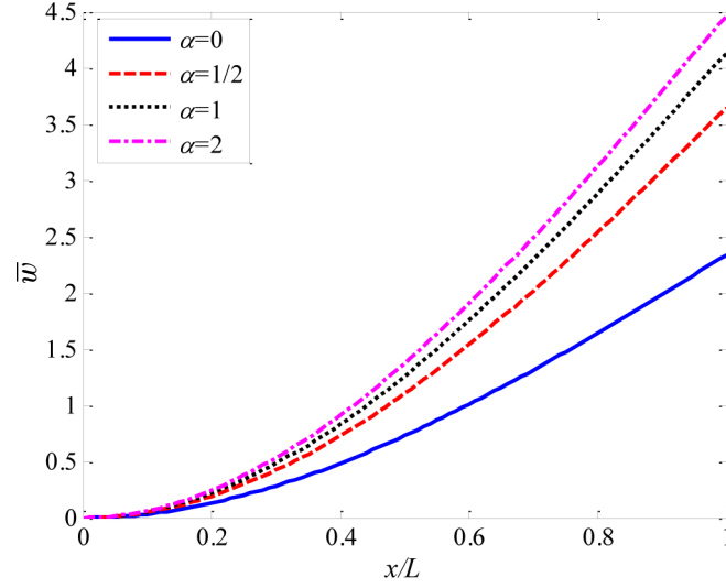
Figure 4. Nondimensional vertical deflection along the beam length for different pressure distribution laws. The nondimensional normal load used in calculation is \bar{F} = 3 .
