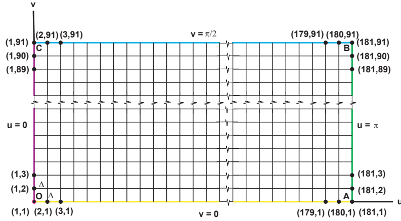
Figure 4. Square finite difference grid map of the curvilinear orthogonal coordinate system.
