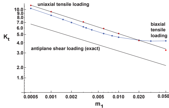
Figure 9. Stress concentration factor versus elliptic integral parameter.
