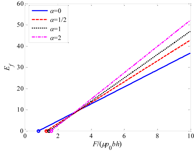
Figure 6. Nondimensional energy dissipation as a function of nondimensional normal load for different pressure distribution laws. The symbols \bigcirc is for the minimum force values inducing relative slip.
