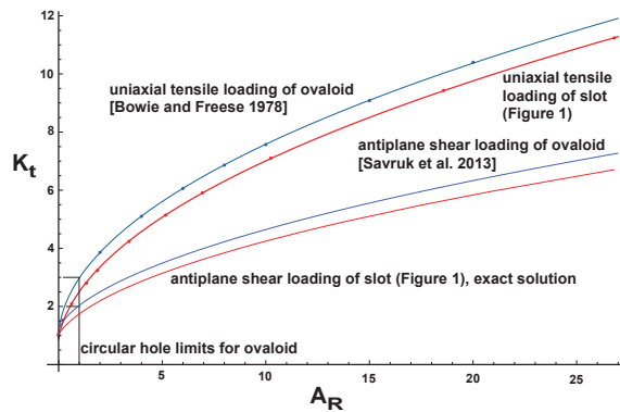
Figure 10. Comparison of stress concentration factor versus aspect ratio for two elongated holes.
