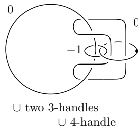
Figure 11. Handlebody structure of a neighborhood of S^2 in S^4 .
