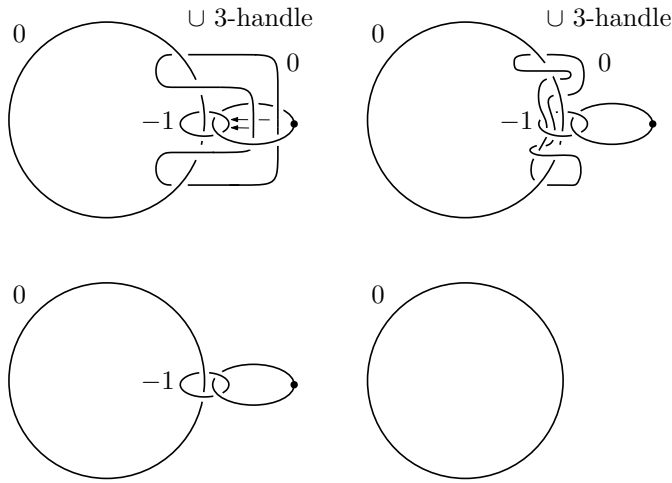
Figure 8. Sliding handles in the concave fibration to identify canceling pairs. After sliding one of the 0-framed 2-handles over the (-1) -framed 2-handle H_2 twice, the slid handle becomes a 0-framed unknot that can be canceled with the 3-handle. The handle H_2 can then be canceled with the 1-handle, leaving behind S^2 \times D^2 .
